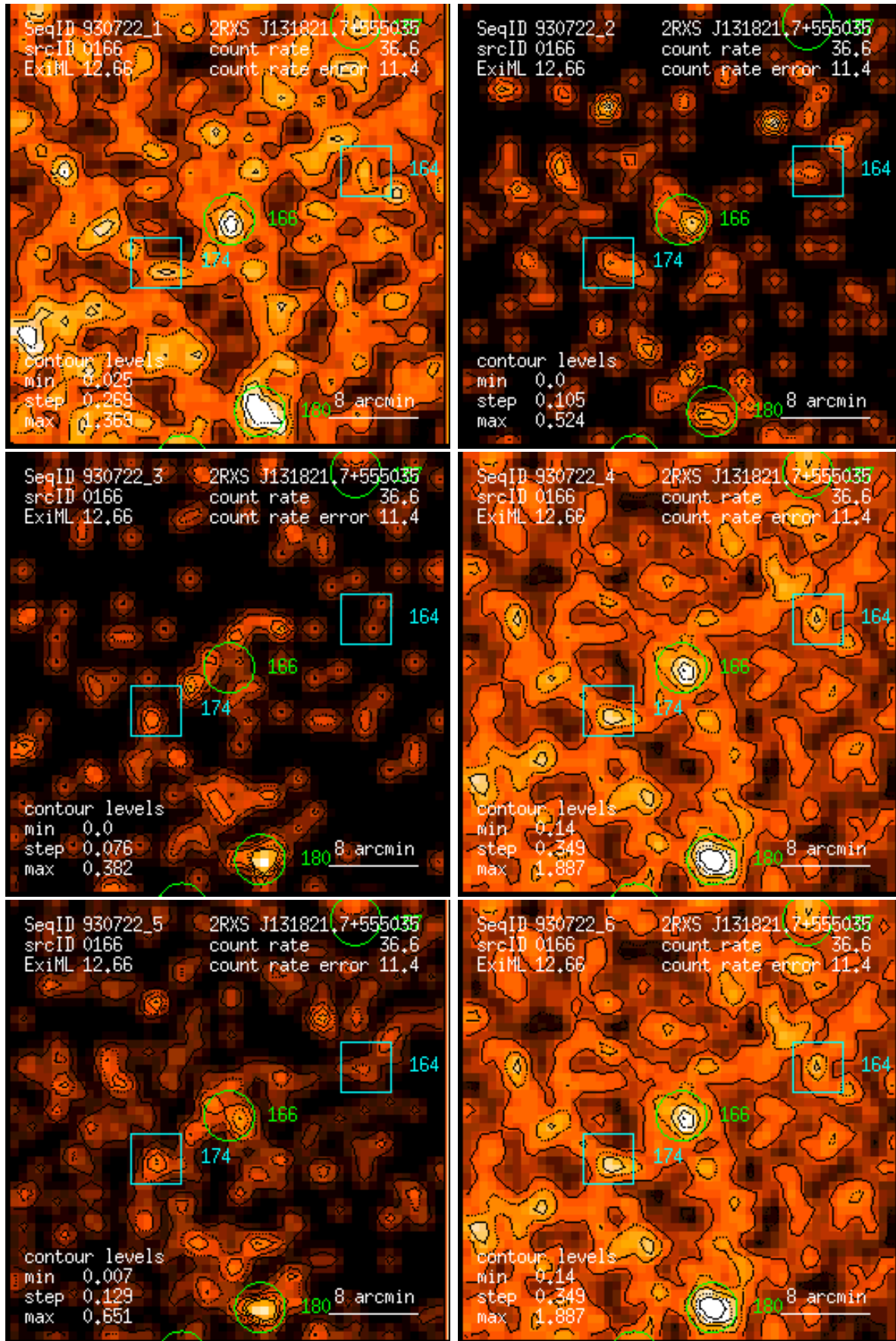
Figure 166: RASS 930722: detection 0166: band rate images, Gaussian filter: (1) PSPC channels 11 – 41, (2) 52 – 90, (3) 91 – 201, (4) 11 – 235, (5) 52 – 201, (6) 11 – 201. Broad band rates in counts/ks. Band rate contour levels in counts/ks/arcmin 2 .
