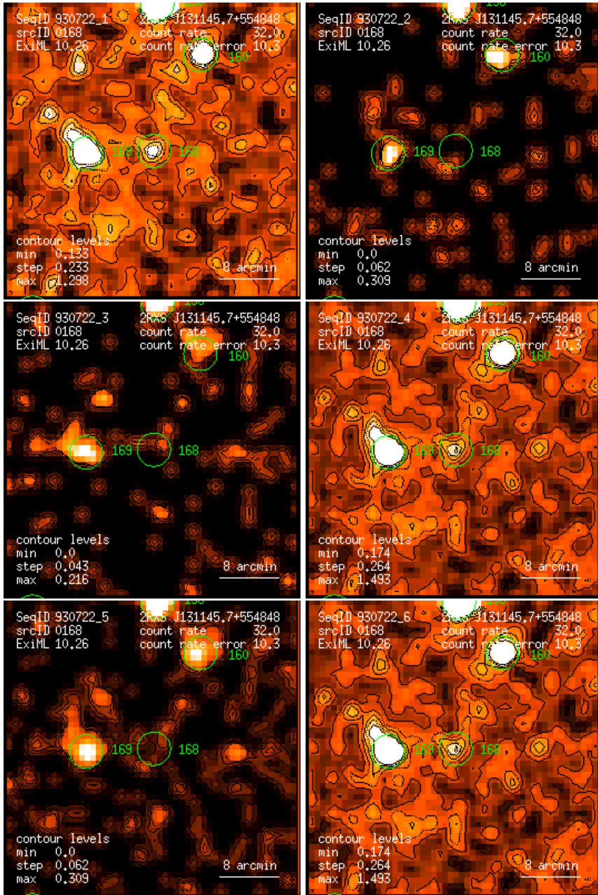
Figure 168: RASS 930722: detection 0168: band rate images, Gaussian filter: (1) PSPC channels 11 – 41, (2) 52 – 90, (3) 91 – 201, (4) 11 – 235, (5) 52 – 201, (6) 11 – 201. Broad band rates in counts/ks. Band rate contour levels in counts/ks/arcmin 2 .
