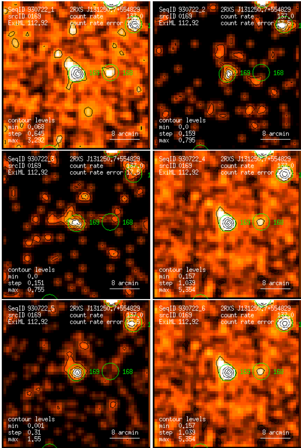
Figure 169: RASS 930722: detection 0169: band rate images, Gaussian filter: (1) PSPC channels 11 – 41, (2) 52 – 90, (3) 91 – 201, (4) 11 – 235, (5) 52 – 201, (6) 11 – 201. Broad band rates in counts/ks. Band rate contour levels in counts/ks/arcmin 2 .
