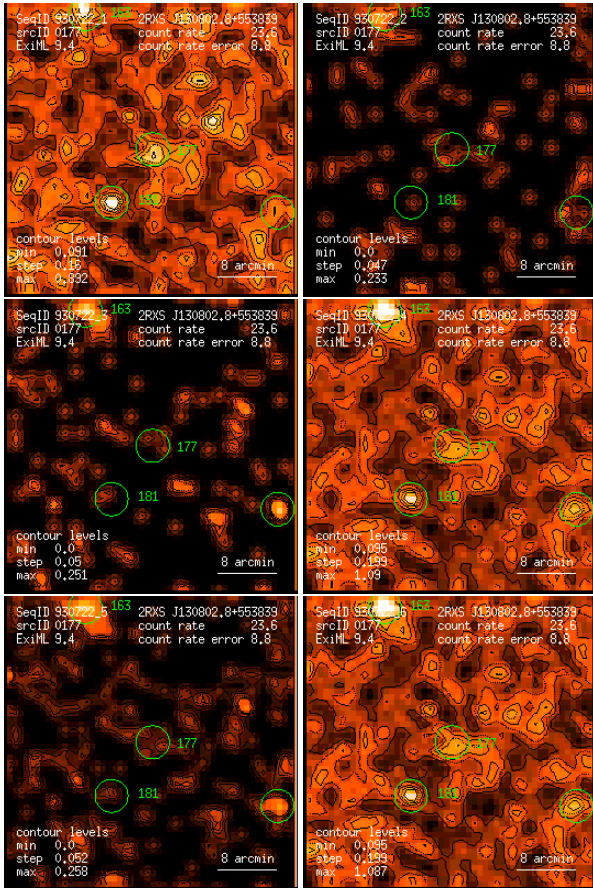
Figure 177: RASS 930722: detection 0177: band rate images, Gaussian filter: (1) PSPC channels 11 – 41, (2) 52 – 90, (3) 91 – 201, (4) 11 – 235, (5) 52 – 201, (6) 11 – 201. Broad band rates in counts/ks. Band rate contour levels in counts/ks/arcmin 2 .
