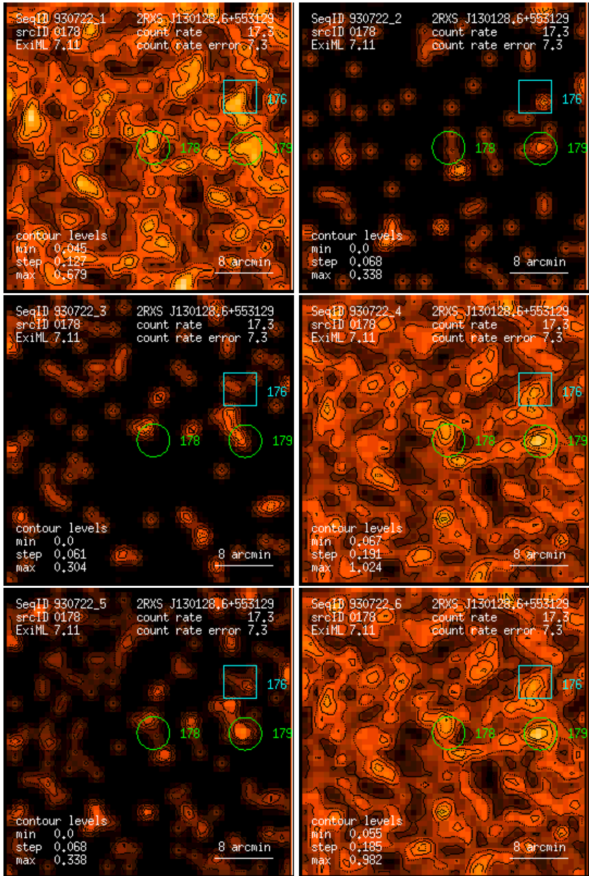
Figure 178: RASS 930722: detection 0178: band rate images, Gaussian filter: (1) PSPC channels 11 – 41, (2) 52 – 90, (3) 91 – 201, (4) 11 – 235, (5) 52 – 201, (6) 11 – 201. Broad band rates in counts/ks. Band rate contour levels in counts/ks/arcmin 2 .
