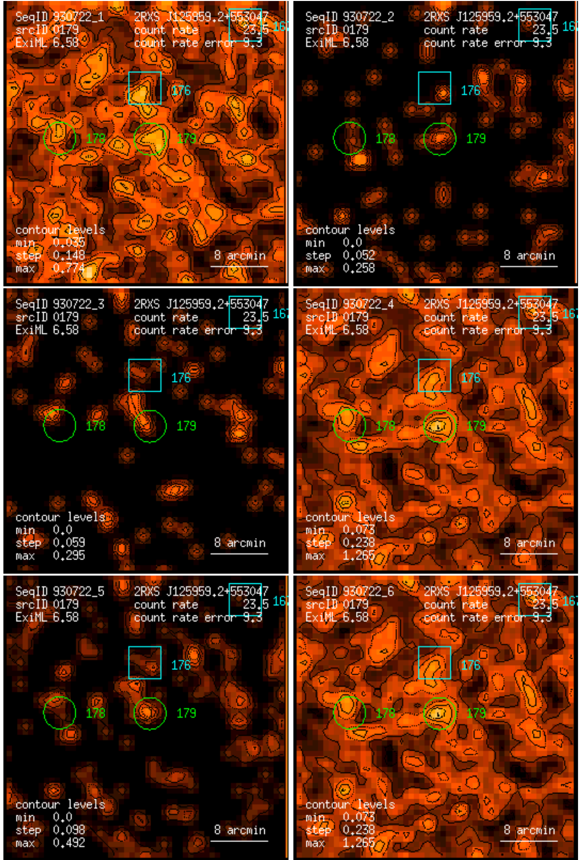
Figure 179: RASS 930722: detection 0179: band rate images, Gaussian filter: (1) PSPC channels 11 – 41, (2) 52 – 90, (3) 91 – 201, (4) 11 – 235, (5) 52 – 201, (6) 11 – 201. Broad band rates in counts/ks. Band rate contour levels in counts/ks/arcmin 2 .
