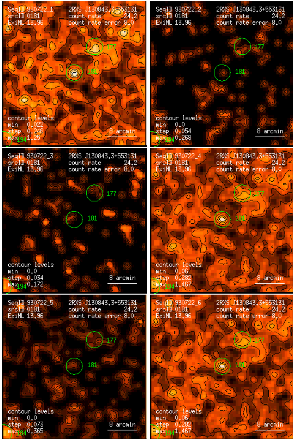
Figure 181: RASS 930722: detection 0181: band rate images, Gaussian filter: (1) PSPC channels 11 – 41, (2) 52 – 90, (3) 91 – 201, (4) 11 – 235, (5) 52 – 201, (6) 11 – 201. Broad band rates in counts/ks. Band rate contour levels in counts/ks/arcmin 2 .
