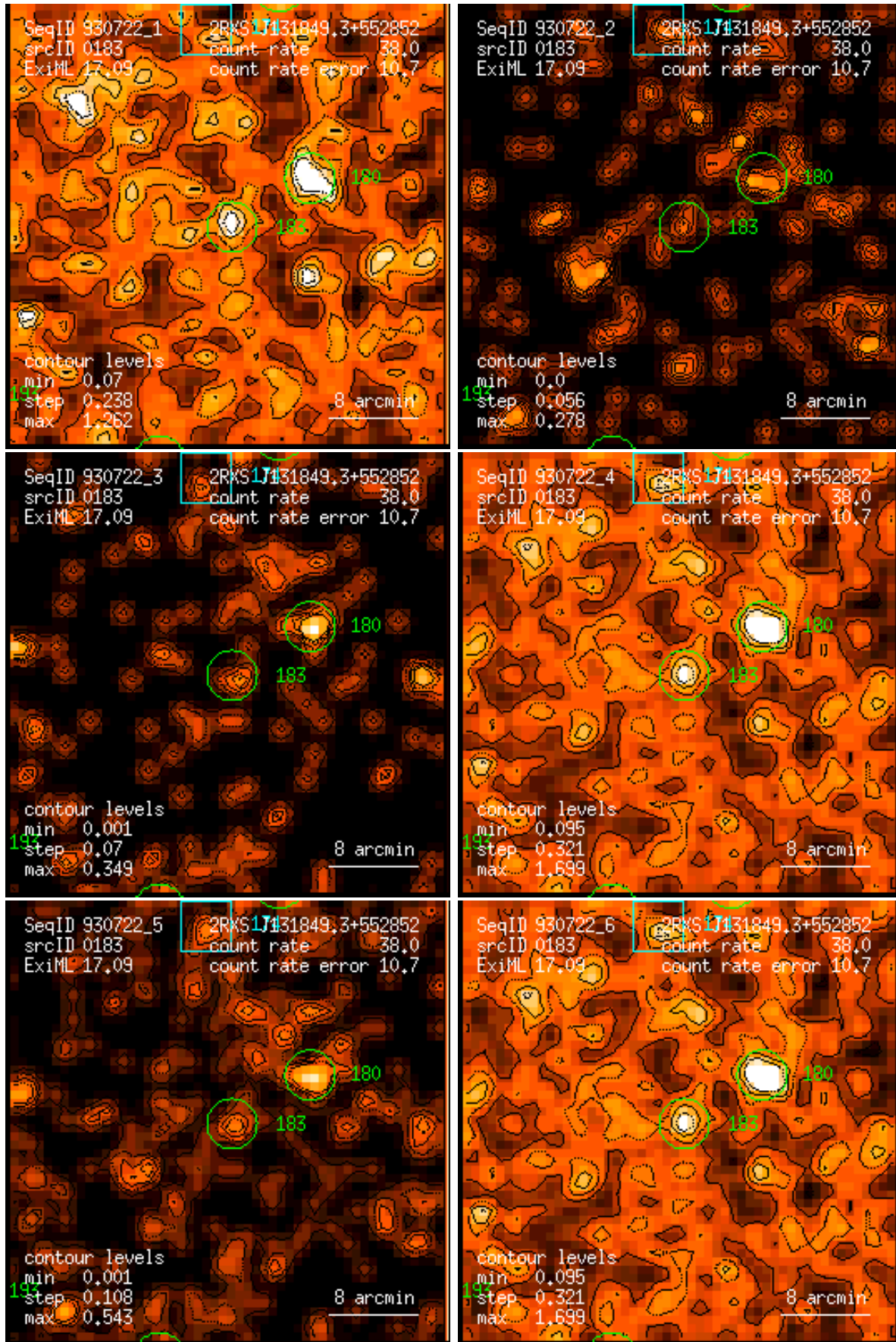
Figure 183: RASS 930722: detection 0183: band rate images, Gaussian filter: (1) PSPC channels 11 – 41, (2) 52 – 90, (3) 91 – 201, (4) 11 – 235, (5) 52 – 201, (6) 11 – 201. Broad band rates in counts/ks. Band rate contour levels in counts/ks/arcmin 2 .
