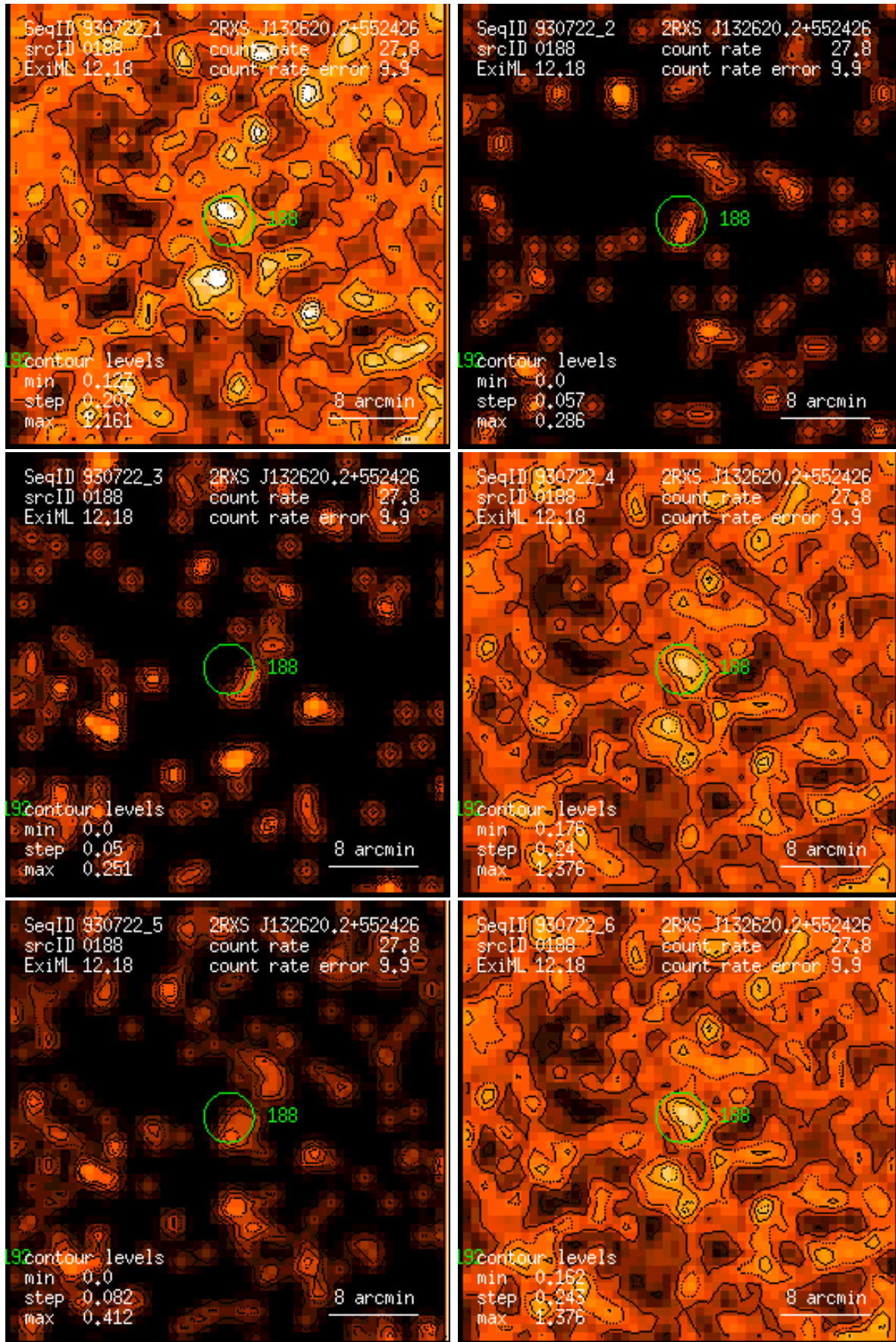
Figure 188: RASS 930722: detection 0188: band rate images, Gaussian filter: (1) PSPC channels 11 – 41, (2) 52 – 90, (3) 91 – 201, (4) 11 – 235, (5) 52 – 201, (6) 11 – 201. Broad band rates in counts/ks. Band rate contour levels in counts/ks/arcmin 2 .
