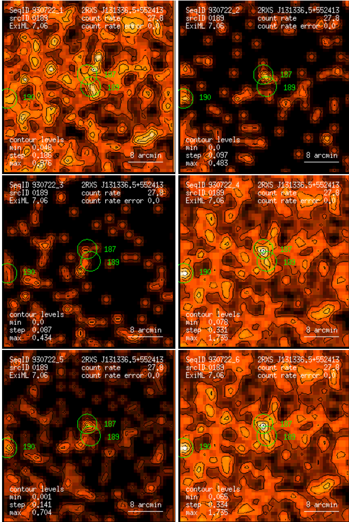
Figure 189: RASS 930722: detection 0189: band rate images, Gaussian filter: (1) PSPC channels 11 – 41, (2) 52 – 90, (3) 91 – 201, (4) 11 – 235, (5) 52 – 201, (6) 11 – 201. Broad band rates in counts/ks. Band rate contour levels in counts/ks/arcmin 2 .
