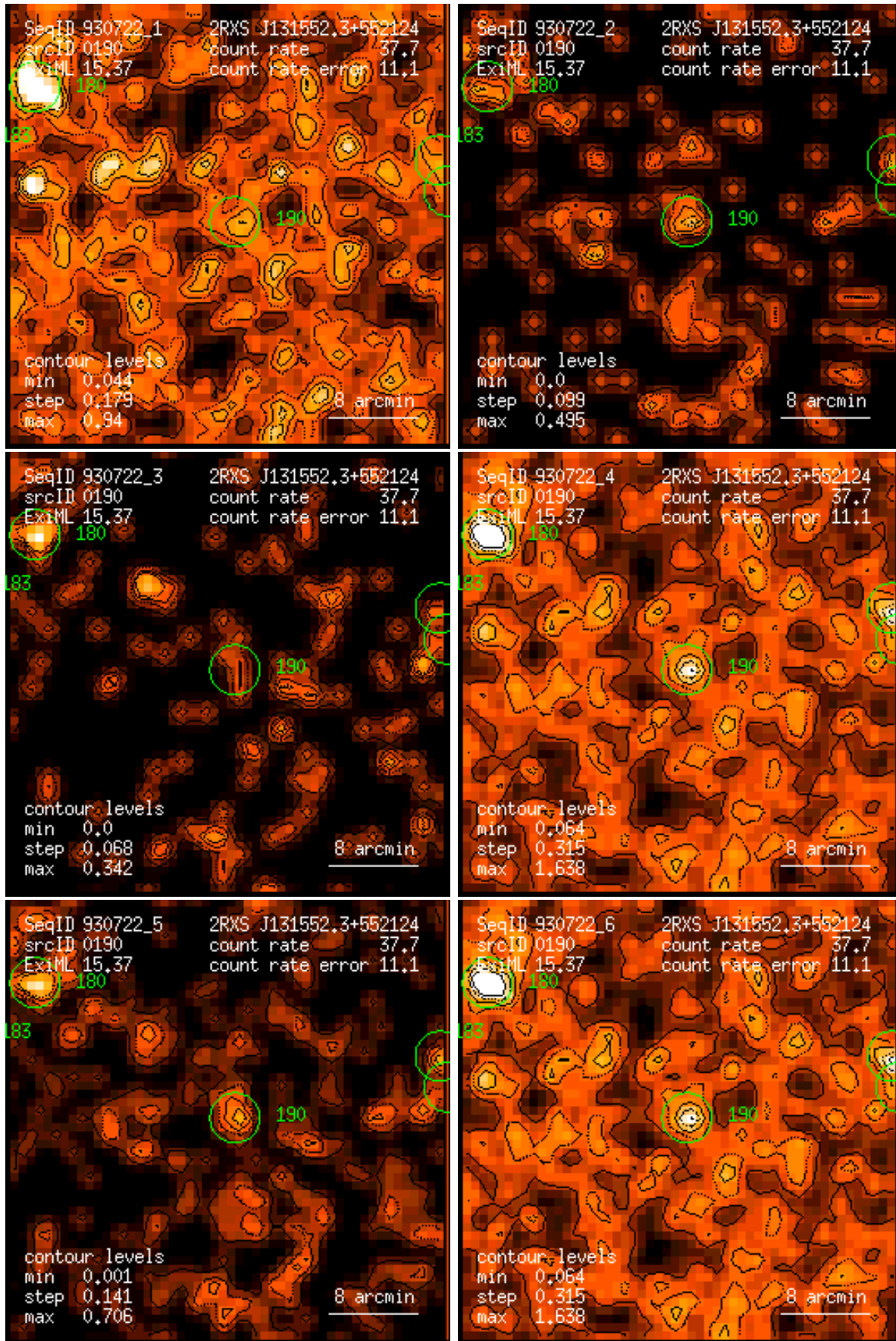
Figure 190: RASS 930722: detection 0190: band rate images, Gaussian filter: (1) PSPC channels 11 – 41, (2) 52 – 90, (3) 91 – 201, (4) 11 – 235, (5) 52 – 201, (6) 11 – 201. Broad band rates in counts/ks. Band rate contour levels in counts/ks/arcmin 2 .
