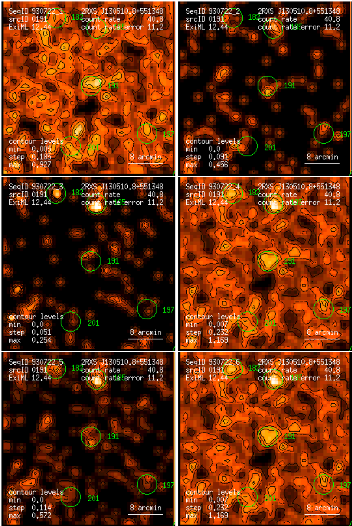
Figure 191: RASS 930722: detection 0191: band rate images, Gaussian filter: (1) PSPC channels 11 – 41, (2) 52 – 90, (3) 91 – 201, (4) 11 – 235, (5) 52 – 201, (6) 11 – 201. Broad band rates in counts/ks. Band rate contour levels in counts/ks/arcmin 2 .
