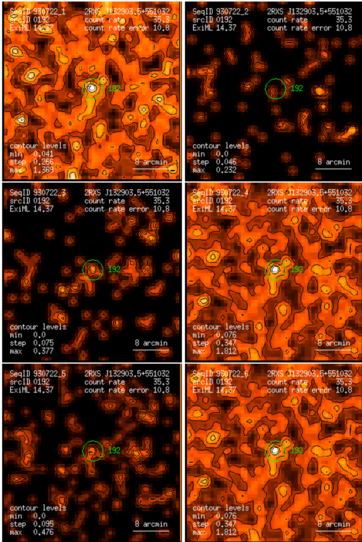
Figure 192: RASS 930722: detection 0192: band rate images, Gaussian filter: (1) PSPC channels 11 – 41, (2) 52 – 90, (3) 91 – 201, (4) 11 – 235, (5) 52 – 201, (6) 11 – 201. Broad band rates in counts/ks. Band rate contour levels in counts/ks/arcmin 2 .
