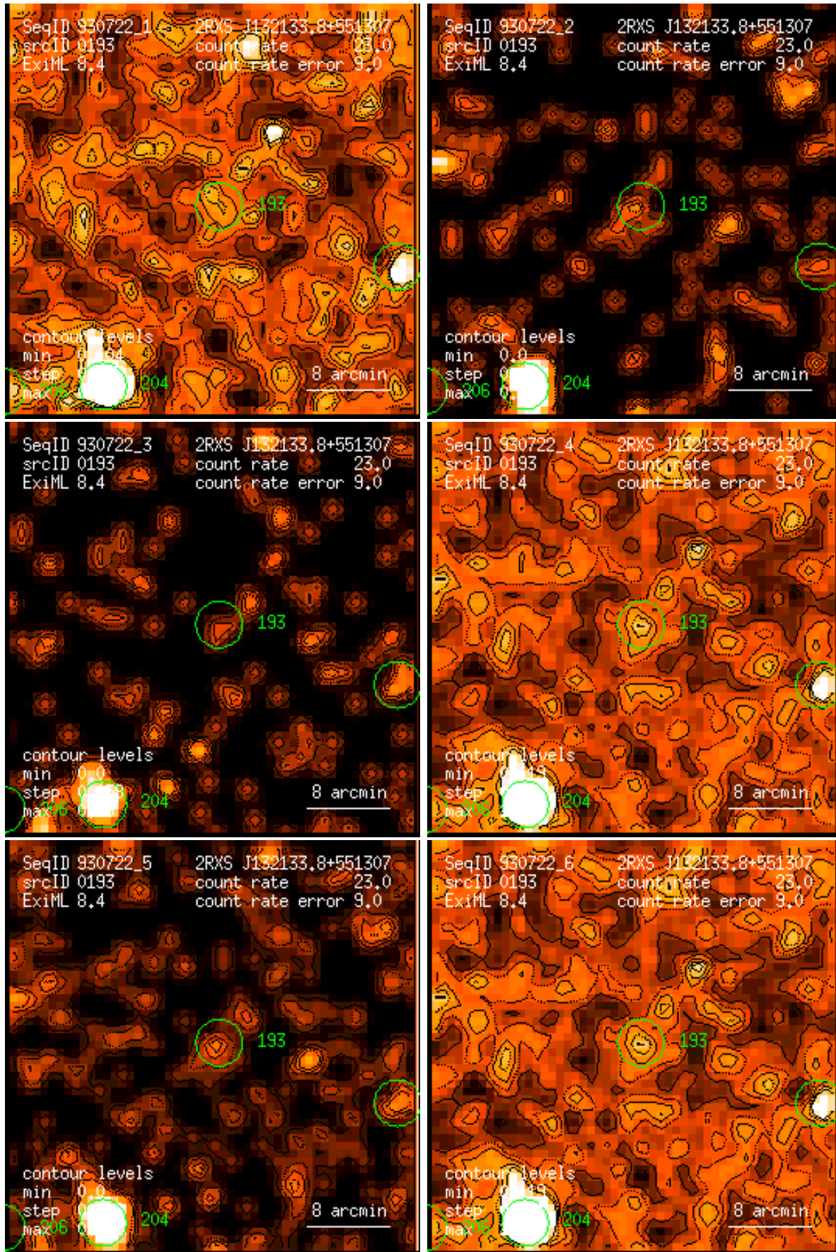
Figure 193: RASS 930722: detection 0193: band rate images, Gaussian filter: (1) PSPC channels 11 – 41, (2) 52 – 90, (3) 91 – 201, (4) 11 – 235, (5) 52 – 201, (6) 11 – 201. Broad band rates in counts/ks. Band rate contour levels in counts/ks/arcmin 2 .
