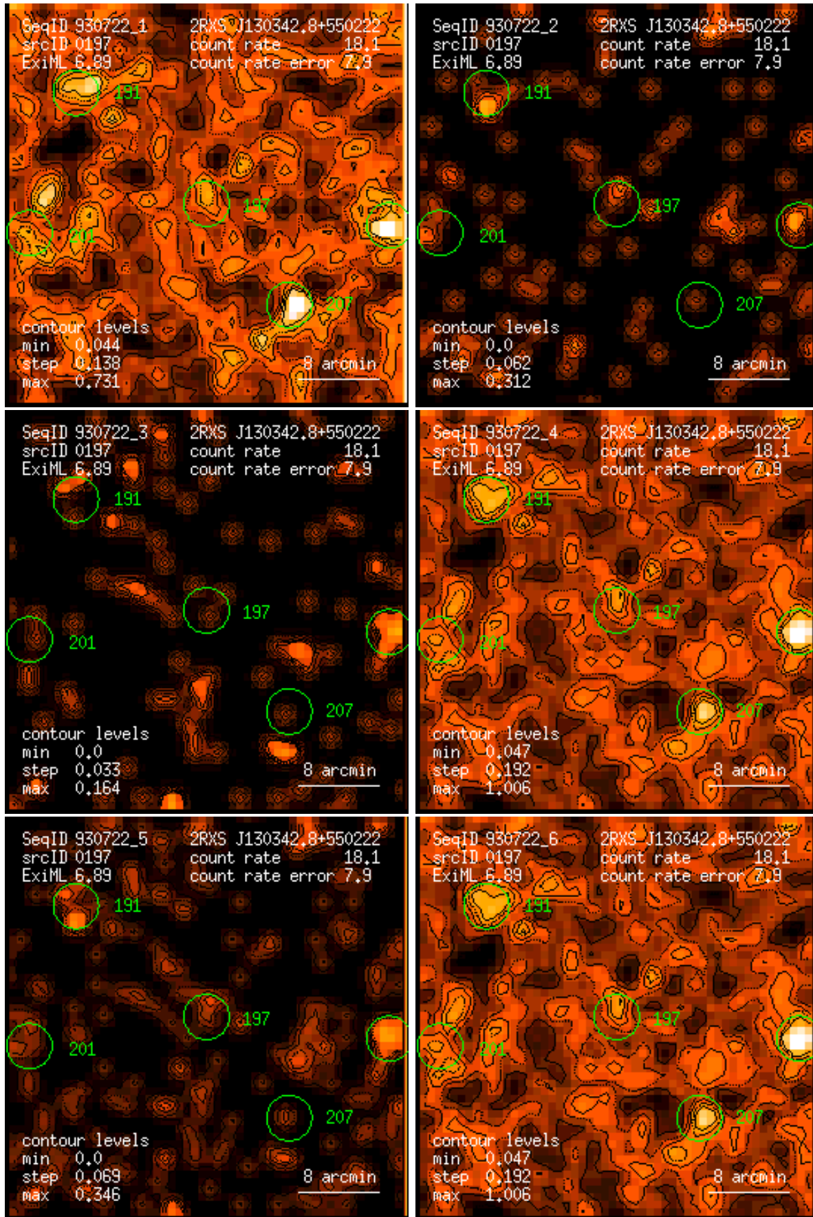
Figure 197: RASS 930722: detection 0197: band rate images, Gaussian filter: (1) PSPC channels 11 – 41, (2) 52 – 90, (3) 91 – 201, (4) 11 – 235, (5) 52 – 201, (6) 11 – 201. Broad band rates in counts/ks. Band rate contour levels in counts/ks/arcmin 2 .
