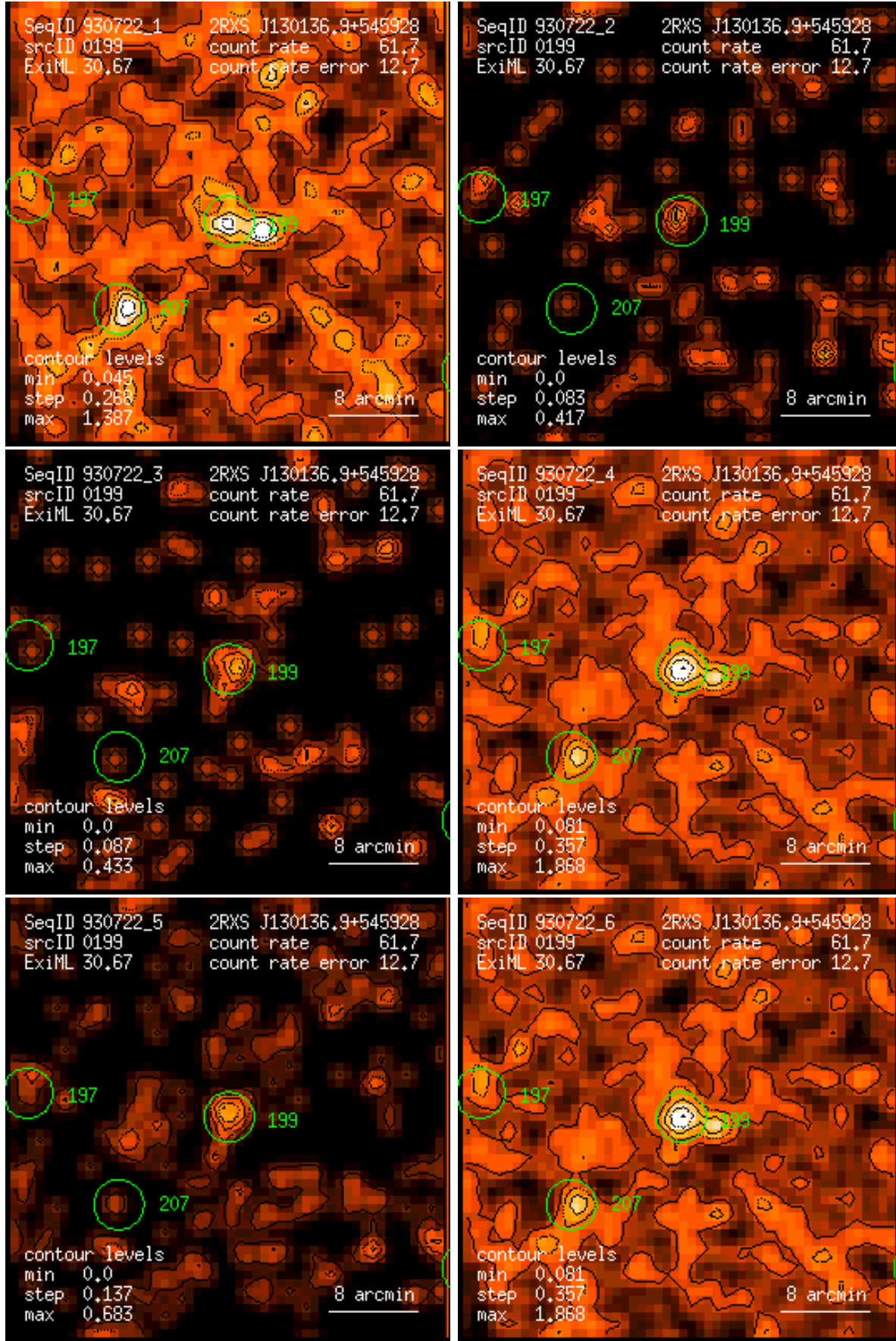
Figure 199: RASS 930722: detection 0199: band rate images, Gaussian filter: (1) PSPC channels 11 – 41, (2) 52 – 90, (3) 91 – 201, (4) 11 – 235, (5) 52 – 201, (6) 11 – 201. Broad band rates in counts/ks. Band rate contour levels in counts/ks/arcmin 2 .
