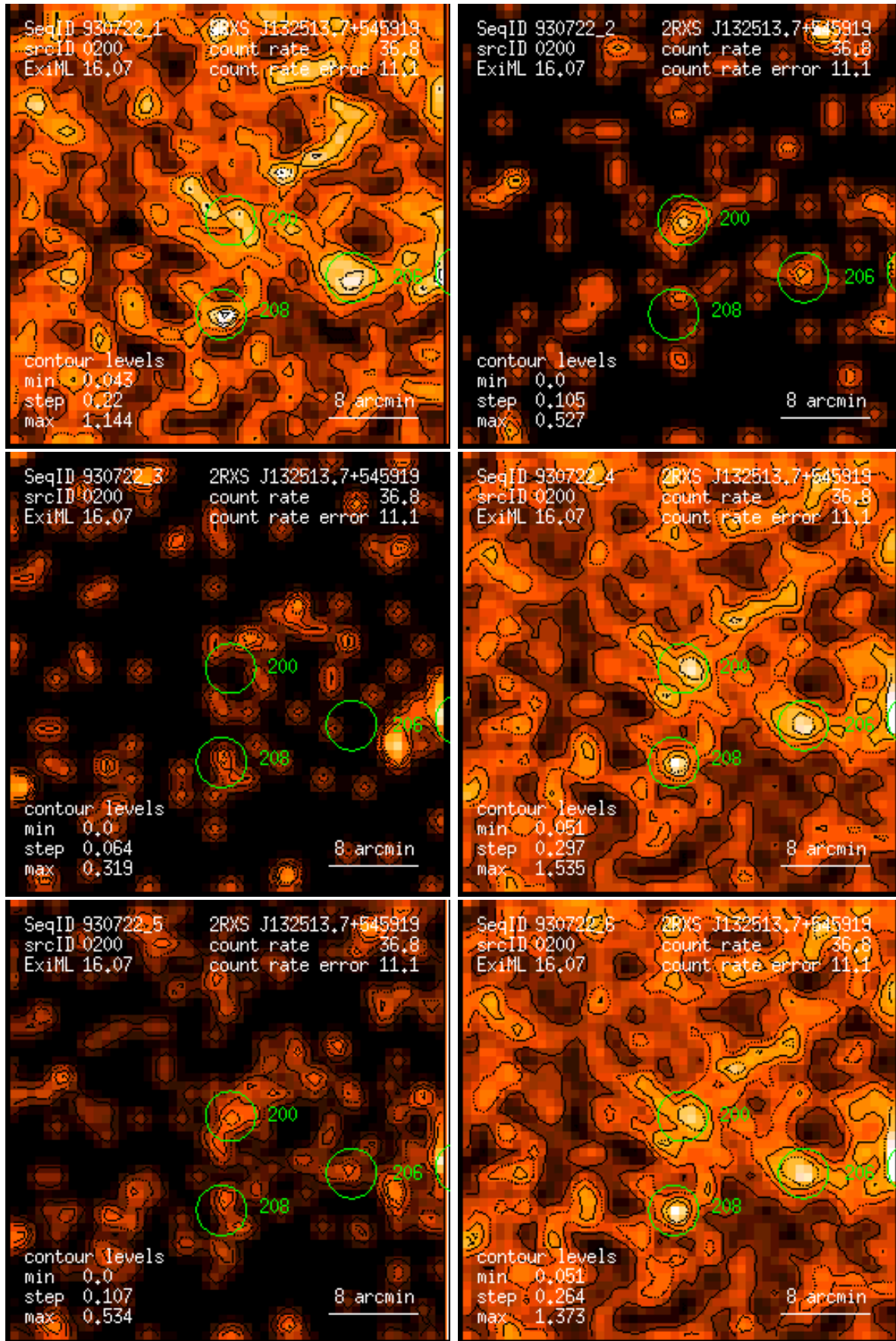
Figure 200: RASS 930722: detection 0200: band rate images, Gaussian filter: (1) PSPC channels 11 – 41, (2) 52 – 90, (3) 91 – 201, (4) 11 – 235, (5) 52 – 201, (6) 11 – 201. Broad band rates in counts/ks. Band rate contour levels in counts/ks/arcmin 2 .
