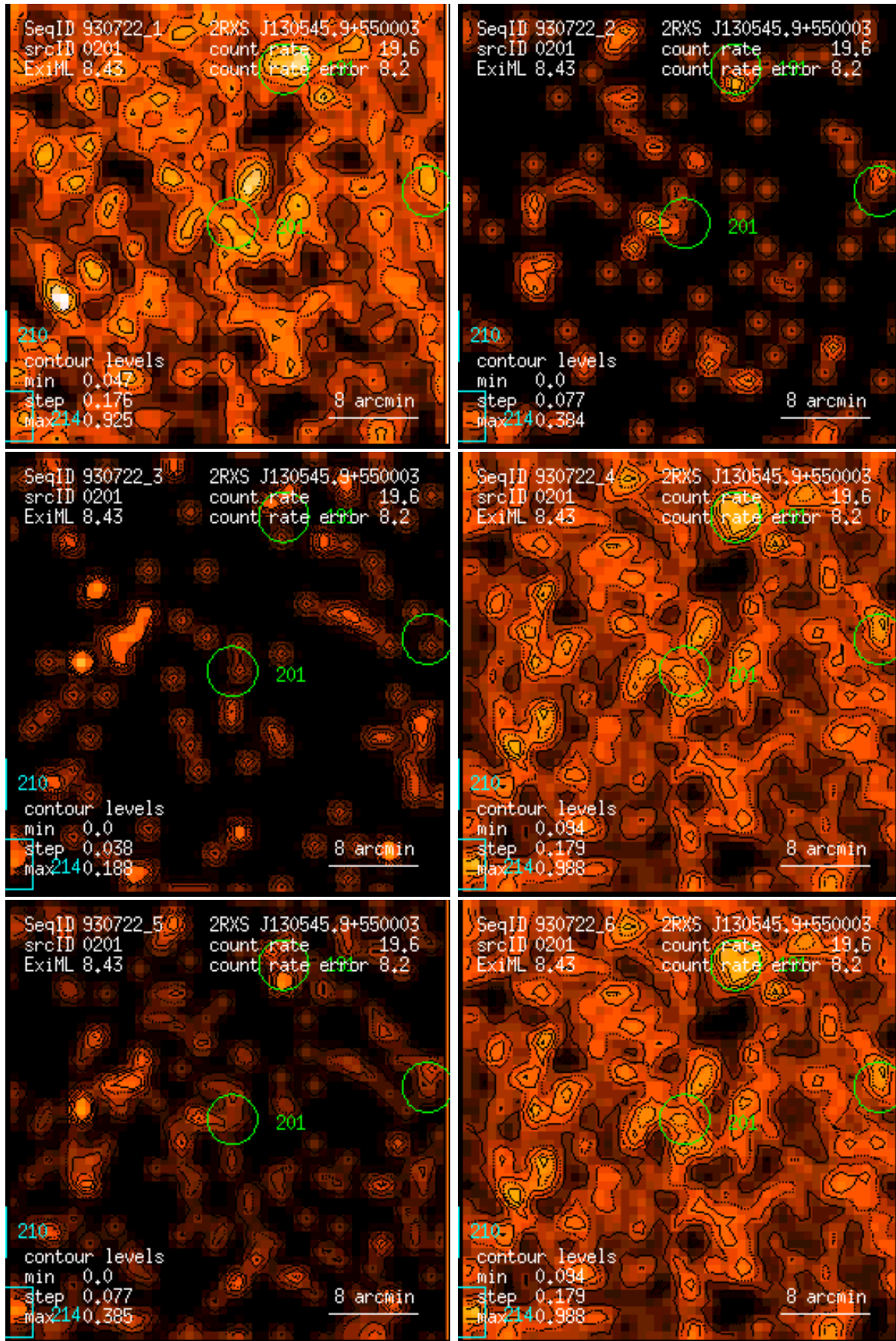
Figure 201: RASS 930722: detection 0201: band rate images, Gaussian filter: (1) PSPC channels 11 – 41, (2) 52 – 90, (3) 91 – 201, (4) 11 – 235, (5) 52 – 201, (6) 11 – 201. Broad band rates in counts/ks. Band rate contour levels in counts/ks/arcmin 2 .
