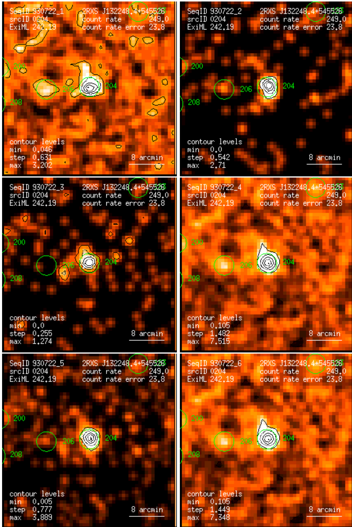
Figure 204: RASS 930722: detection 0204: band rate images, Gaussian filter: (1) PSPC channels 11 – 41, (2) 52 – 90, (3) 91 – 201, (4) 11 – 235, (5) 52 – 201, (6) 11 – 201. Broad band rates in counts/ks. Band rate contour levels in counts/ks/arcmin 2 .
