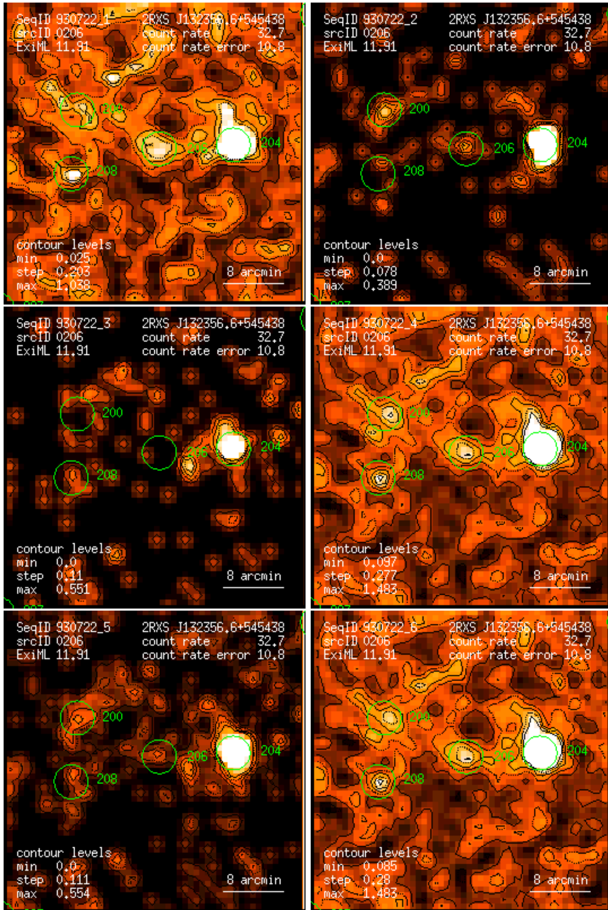
Figure 206: RASS 930722: detection 0206: band rate images, Gaussian filter: (1) PSPC channels 11 – 41, (2) 52 – 90, (3) 91 – 201, (4) 11 – 235, (5) 52 – 201, (6) 11 – 201. Broad band rates in counts/ks. Band rate contour levels in counts/ks/arcmin 2 .
