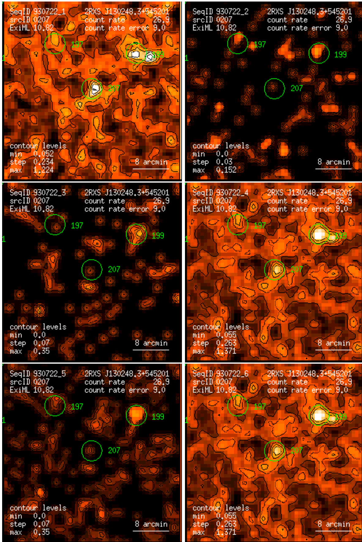
Figure 207: RASS 930722: detection 0207: band rate images, Gaussian filter: (1) PSPC channels 11 – 41, (2) 52 – 90, (3) 91 – 201, (4) 11 – 235, (5) 52 – 201, (6) 11 – 201. Broad band rates in counts/ks. Band rate contour levels in counts/ks/arcmin 2 .
