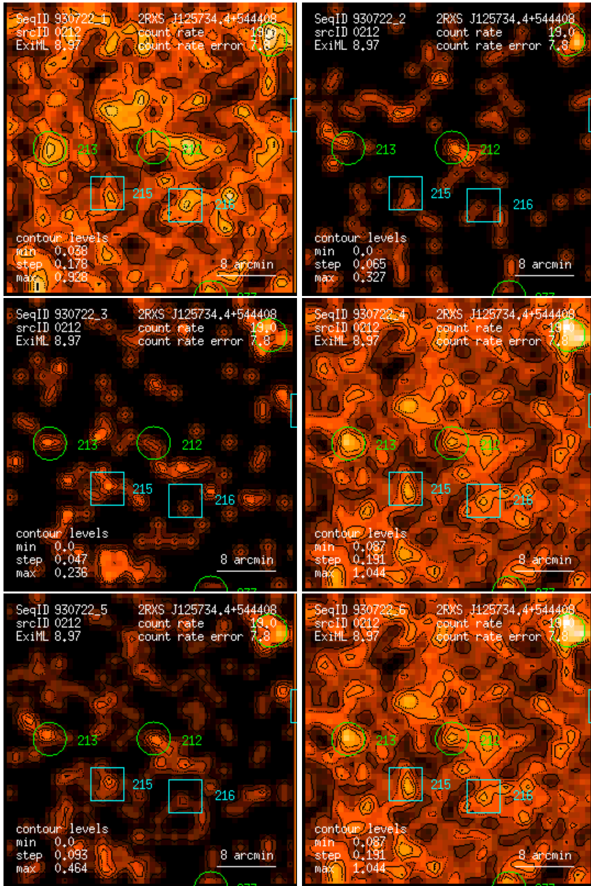
Figure 212: RASS 930722: detection 0212: band rate images, Gaussian filter: (1) PSPC channels 11 – 41, (2) 52 – 90, (3) 91 – 201, (4) 11 – 235, (5) 52 – 201, (6) 11 – 201. Broad band rates in counts/ks. Band rate contour levels in counts/ks/arcmin 2 .
