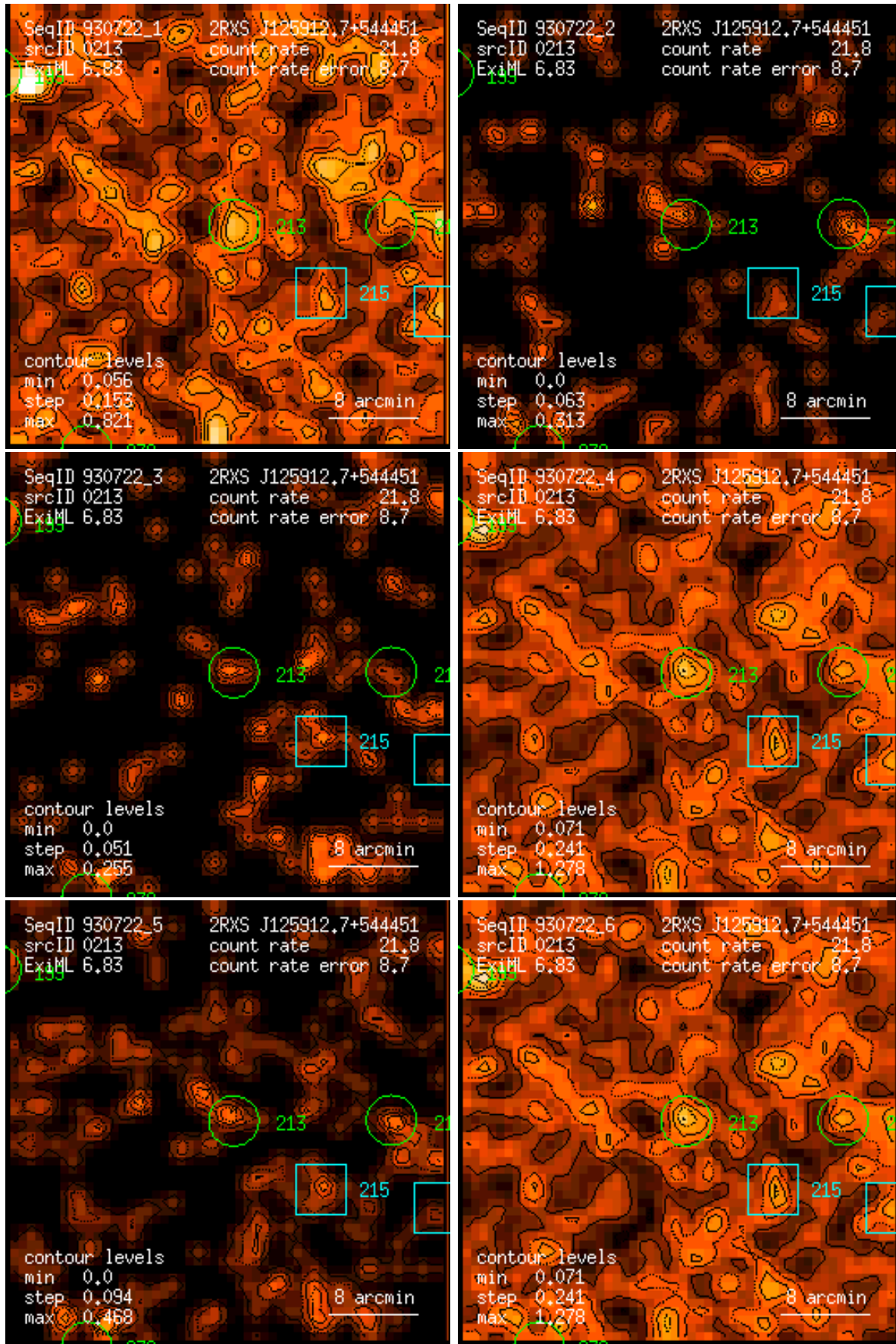
Figure 213: RASS 930722: detection 0213: band rate images, Gaussian filter: (1) PSPC channels 11 – 41, (2) 52 – 90, (3) 91 – 201, (4) 11 – 235, (5) 52 – 201, (6) 11 – 201. Broad band rates in counts/ks. Band rate contour levels in counts/ks/arcmin 2 .
