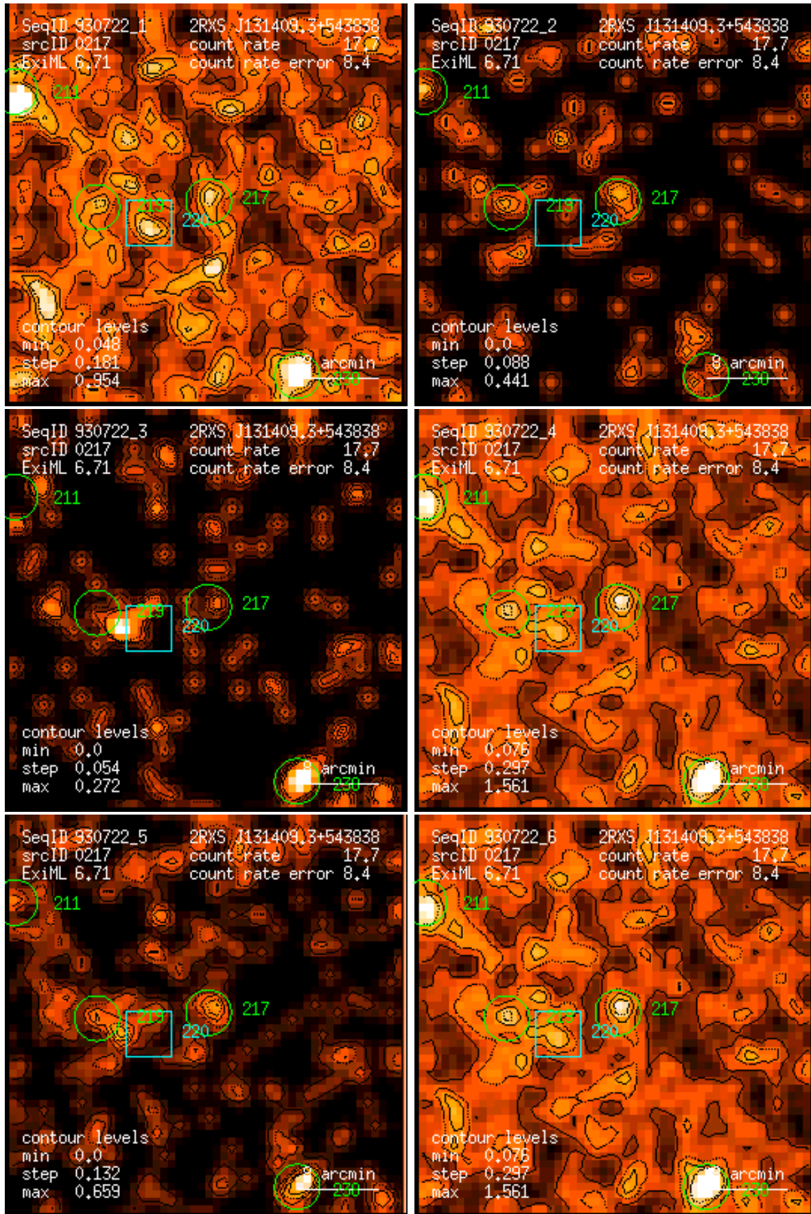
Figure 217: RASS 930722: detection 0217: band rate images, Gaussian filter: (1) PSPC channels 11 – 41, (2) 52 – 90, (3) 91 – 201, (4) 11 – 235, (5) 52 – 201, (6) 11 – 201. Broad band rates in counts/ks. Band rate contour levels in counts/ks/arcmin 2 .
