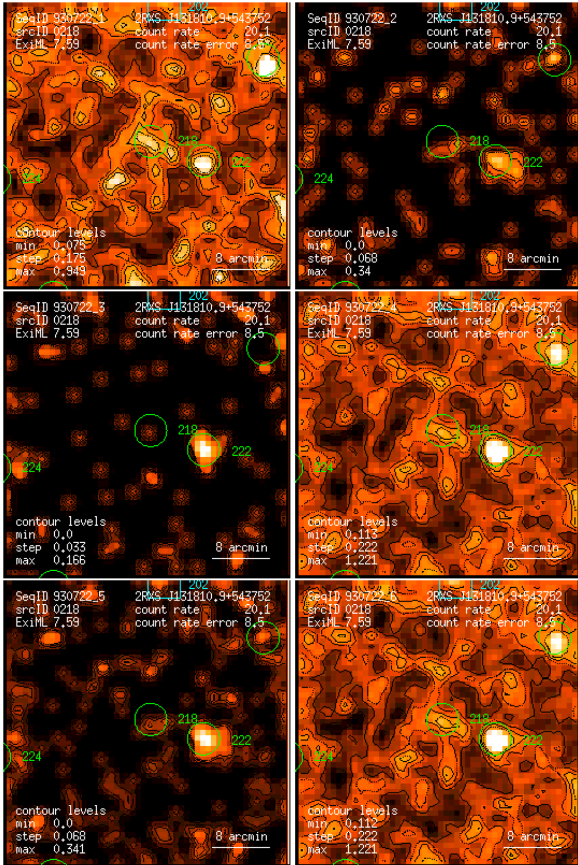
Figure 218: RASS 930722: detection 0218: band rate images, Gaussian filter: (1) PSPC channels 11 – 41, (2) 52 – 90, (3) 91 – 201, (4) 11 – 235, (5) 52 – 201, (6) 11 – 201. Broad band rates in counts/ks. Band rate contour levels in counts/ks/arcmin 2 .
