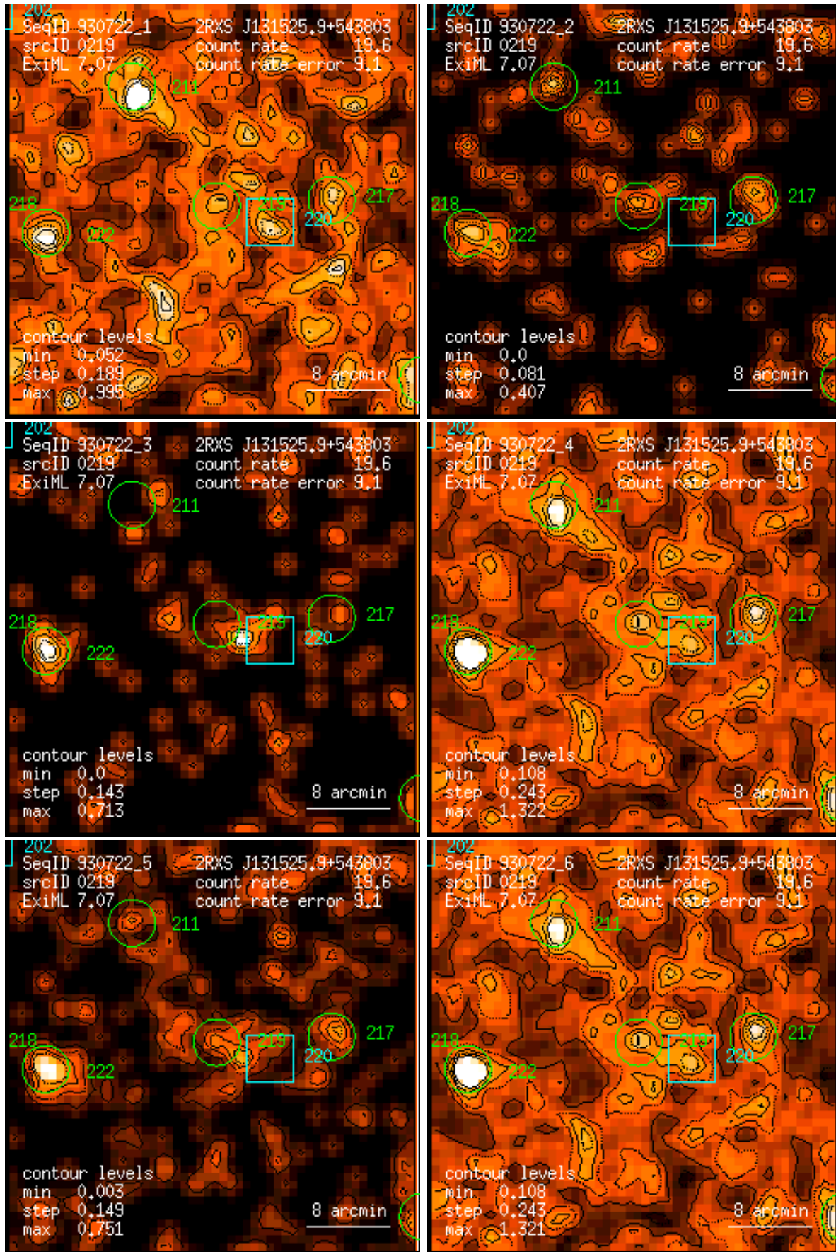
Figure 219: RASS 930722: detection 0219: band rate images, Gaussian filter: (1) PSPC channels 11 – 41, (2) 52 – 90, (3) 91 – 201, (4) 11 – 235, (5) 52 – 201, (6) 11 – 201. Broad band rates in counts/ks. Band rate contour levels in counts/ks/arcmin 2 .
