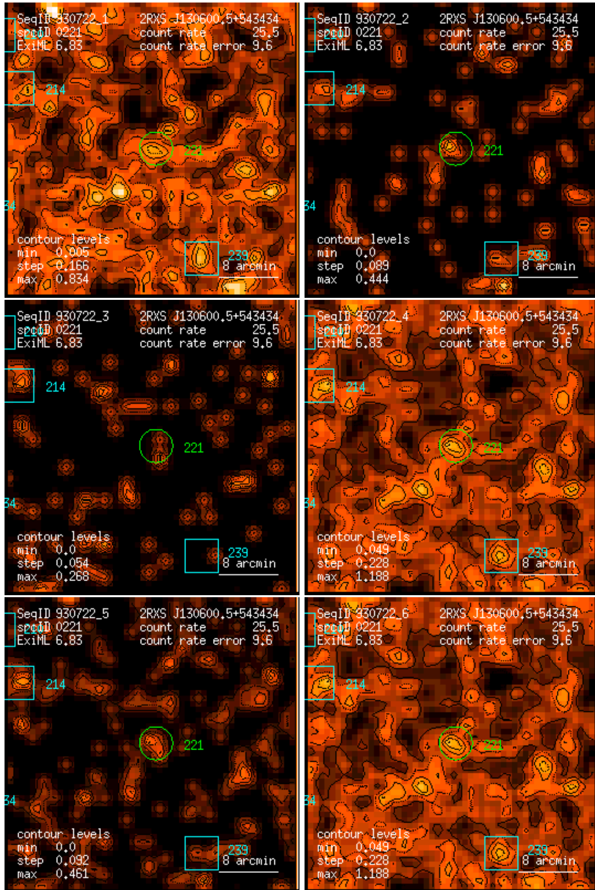
Figure 221: RASS 930722: detection 0221: band rate images, Gaussian filter: (1) PSPC channels 11 – 41, (2) 52 – 90, (3) 91 – 201, (4) 11 – 235, (5) 52 – 201, (6) 11 – 201. Broad band rates in counts/ks. Band rate contour levels in counts/ks/arcmin 2 .
