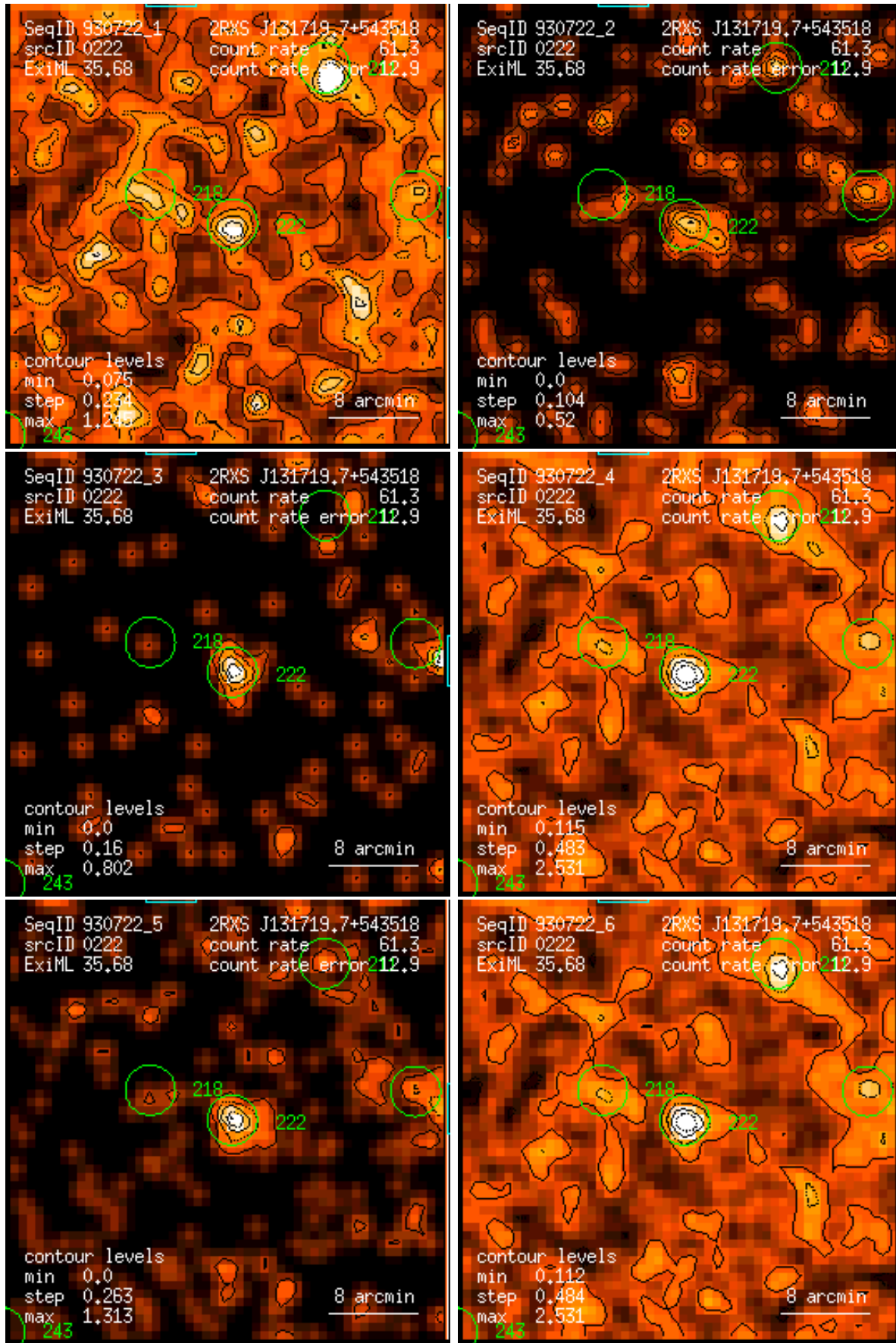
Figure 222: RASS 930722: detection 0222: band rate images, Gaussian filter: (1) PSPC channels 11 – 41, (2) 52 – 90, (3) 91 – 201, (4) 11 – 235, (5) 52 – 201, (6) 11 – 201. Broad band rates in counts/ks. Band rate contour levels in counts/ks/arcmin 2 .
