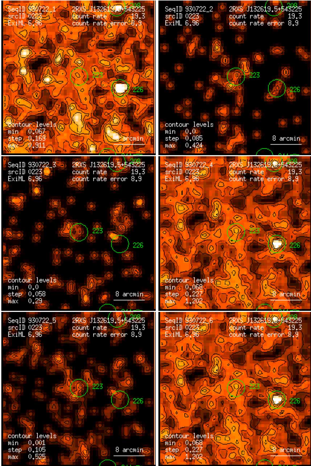
Figure 223: RASS 930722: detection 0223: band rate images, Gaussian filter: (1) PSPC channels 11 – 41, (2) 52 – 90, (3) 91 – 201, (4) 11 – 235, (5) 52 – 201, (6) 11 – 201. Broad band rates in counts/ks. Band rate contour levels in counts/ks/arcmin 2 .
