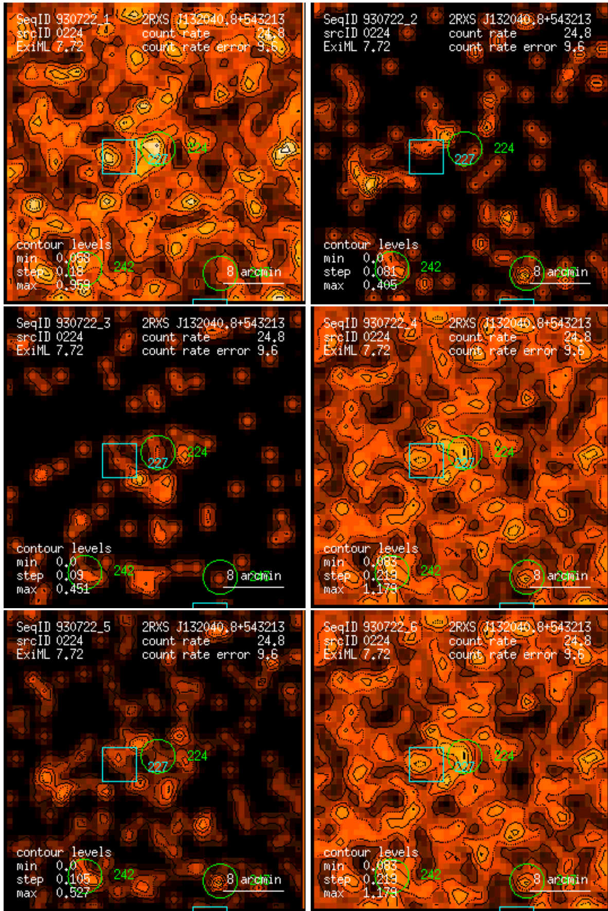
Figure 224: RASS 930722: detection 0224: band rate images, Gaussian filter: (1) PSPC channels 11 – 41, (2) 52 – 90, (3) 91 – 201, (4) 11 – 235, (5) 52 – 201, (6) 11 – 201. Broad band rates in counts/ks. Band rate contour levels in counts/ks/arcmin 2 .
