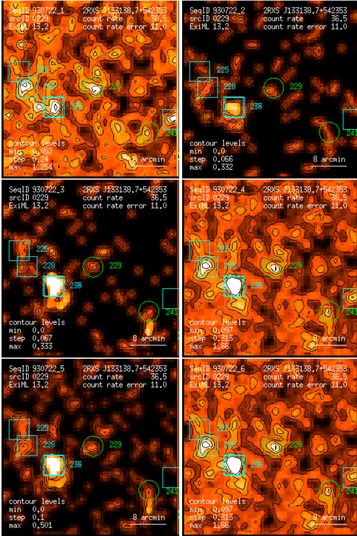
Figure 229: RASS 930722: detection 0229: band rate images, Gaussian filter: (1) PSPC channels 11 – 41, (2) 52 – 90, (3) 91 – 201, (4) 11 – 235, (5) 52 – 201, (6) 11 – 201. Broad band rates in counts/ks. Band rate contour levels in counts/ks/arcmin 2 .
