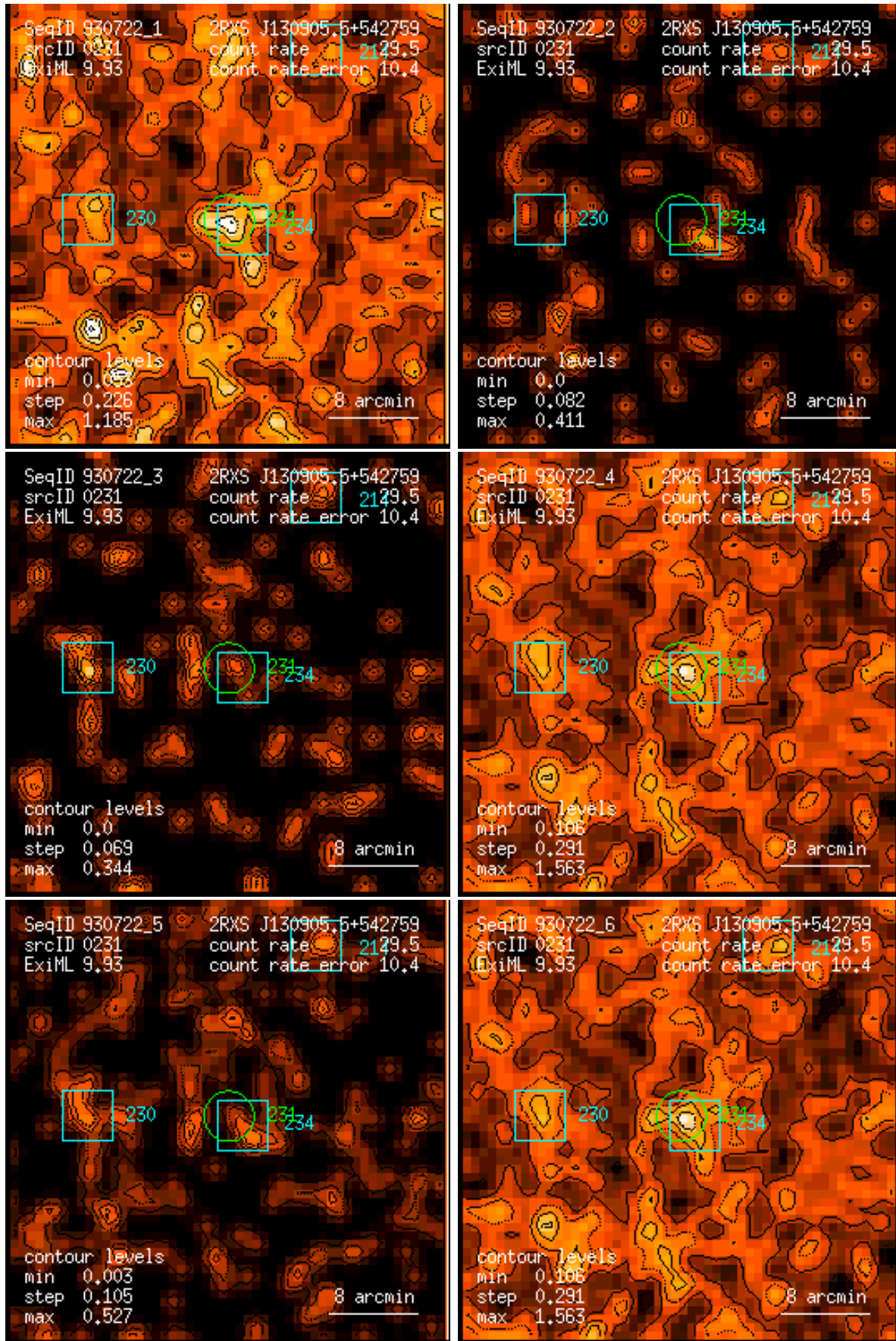
Figure 231: RASS 930722: detection 0231: band rate images, Gaussian filter: (1) PSPC channels 11 – 41, (2) 52 – 90, (3) 91 – 201, (4) 11 – 235, (5) 52 – 201, (6) 11 – 201. Broad band rates in counts/ks. Band rate contour levels in counts/ks/arcmin 2 .
