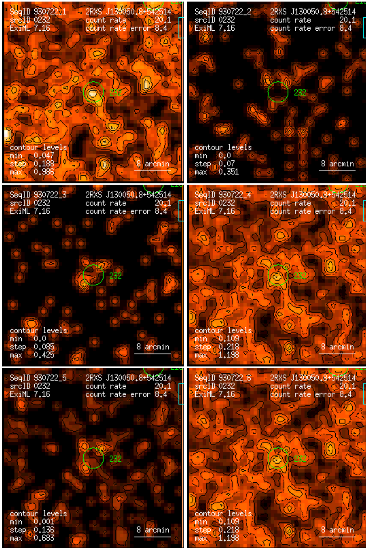
Figure 232: RASS 930722: detection 0232: band rate images, Gaussian filter: (1) PSPC channels 11 – 41, (2) 52 – 90, (3) 91 – 201, (4) 11 – 235, (5) 52 – 201, (6) 11 – 201. Broad band rates in counts/ks. Band rate contour levels in counts/ks/arcmin 2 .
