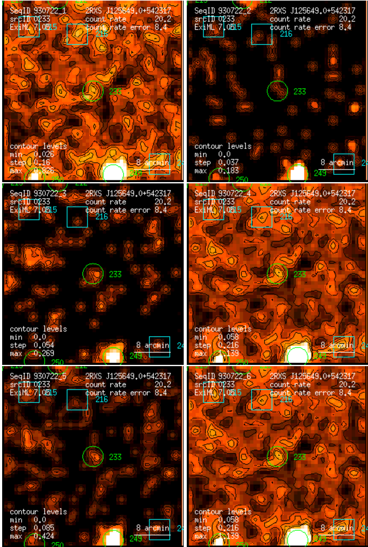
Figure 233: RASS 930722: detection 0233: band rate images, Gaussian filter: (1) PSPC channels 11 – 41, (2) 52 – 90, (3) 91 – 201, (4) 11 – 235, (5) 52 – 201, (6) 11 – 201. Broad band rates in counts/ks. Band rate contour levels in counts/ks/arcmin 2 .
