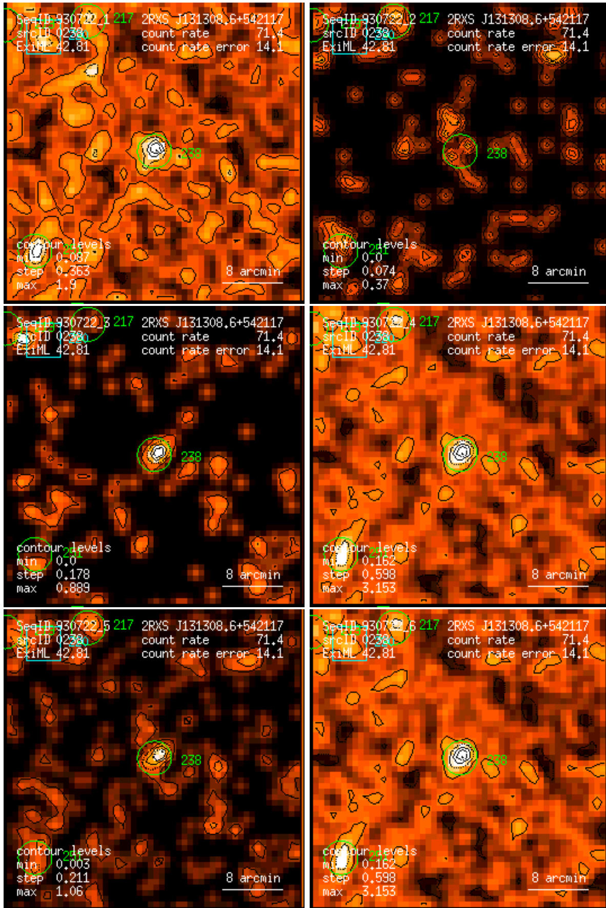
Figure 238: RASS 930722: detection 0238: band rate images, Gaussian filter: (1) PSPC channels 11 – 41, (2) 52 – 90, (3) 91 – 201, (4) 11 – 235, (5) 52 – 201, (6) 11 – 201. Broad band rates in counts/ks. Band rate contour levels in counts/ks/arcmin 2 .
