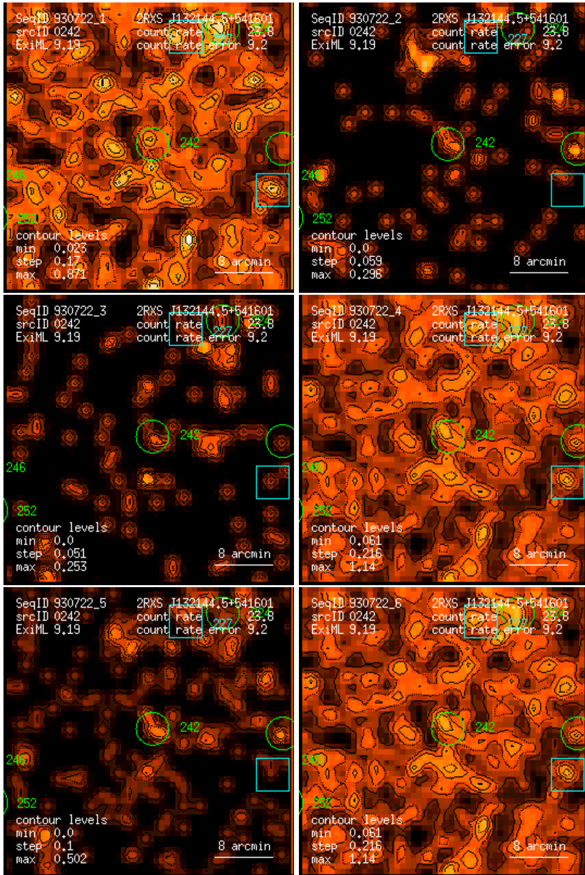
Figure 242: RASS 930722: detection 0242: band rate images, Gaussian filter: (1) PSPC channels 11 – 41, (2) 52 – 90, (3) 91 – 201, (4) 11 – 235, (5) 52 – 201, (6) 11 – 201. Broad band rates in counts/ks. Band rate contour levels in counts/ks/arcmin 2 .
