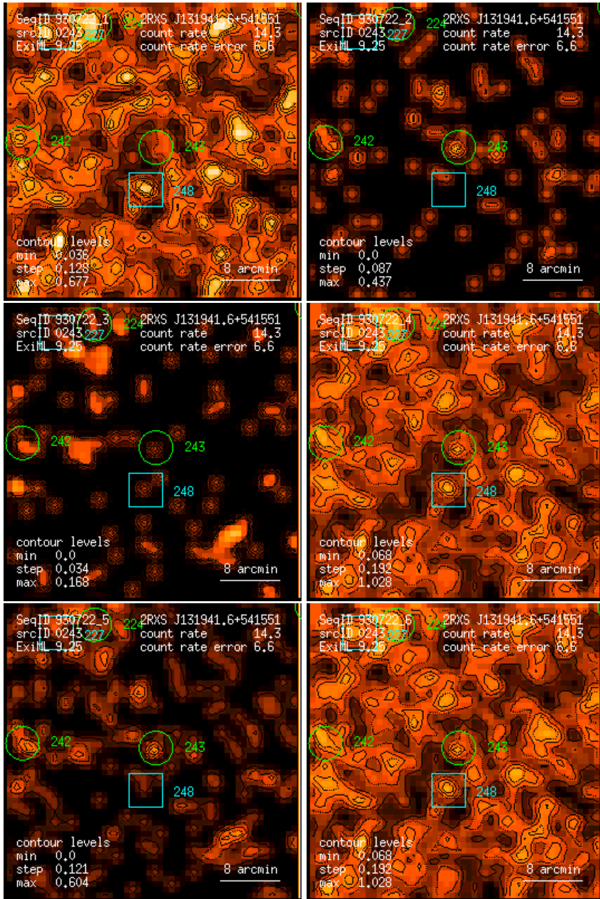
Figure 243: RASS 930722: detection 0243: band rate images, Gaussian filter: (1) PSPC channels 11 – 41, (2) 52 – 90, (3) 91 – 201, (4) 11 – 235, (5) 52 – 201, (6) 11 – 201. Broad band rates in counts/ks. Band rate contour levels in counts/ks/arcmin 2 .
