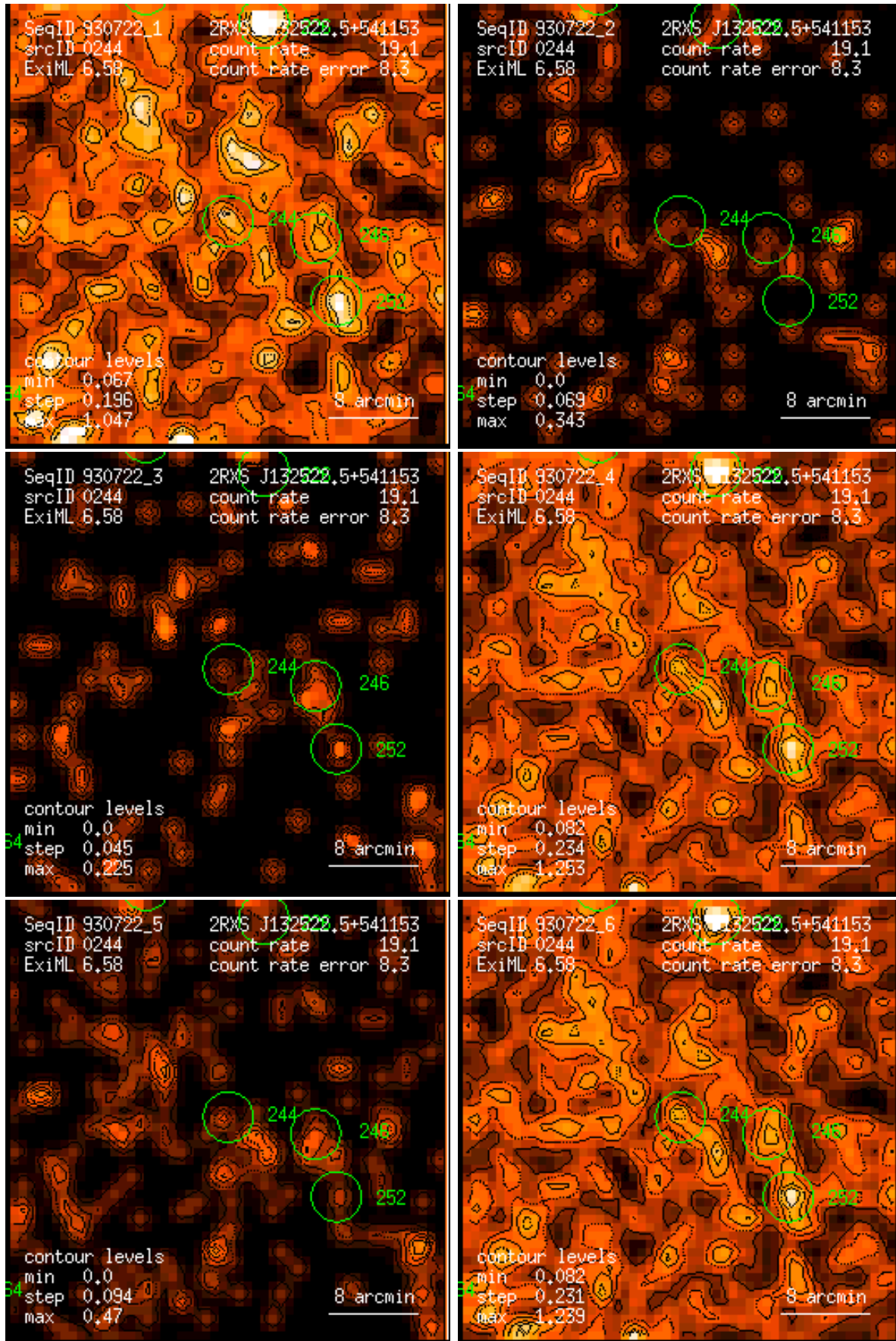
Figure 244: RASS 930722: detection 0244: band rate images, Gaussian filter: (1) PSPC channels 11 – 41, (2) 52 – 90, (3) 91 – 201, (4) 11 – 235, (5) 52 – 201, (6) 11 – 201. Broad band rates in counts/ks. Band rate contour levels in counts/ks/arcmin 2 .
