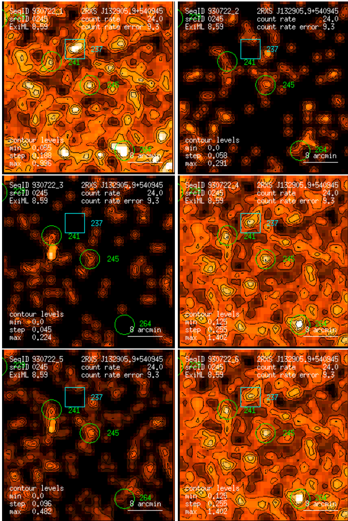
Figure 245: RASS 930722: detection 0245: band rate images, Gaussian filter: (1) PSPC channels 11 – 41, (2) 52 – 90, (3) 91 – 201, (4) 11 – 235, (5) 52 – 201, (6) 11 – 201. Broad band rates in counts/ks. Band rate contour levels in counts/ks/arcmin 2 .
