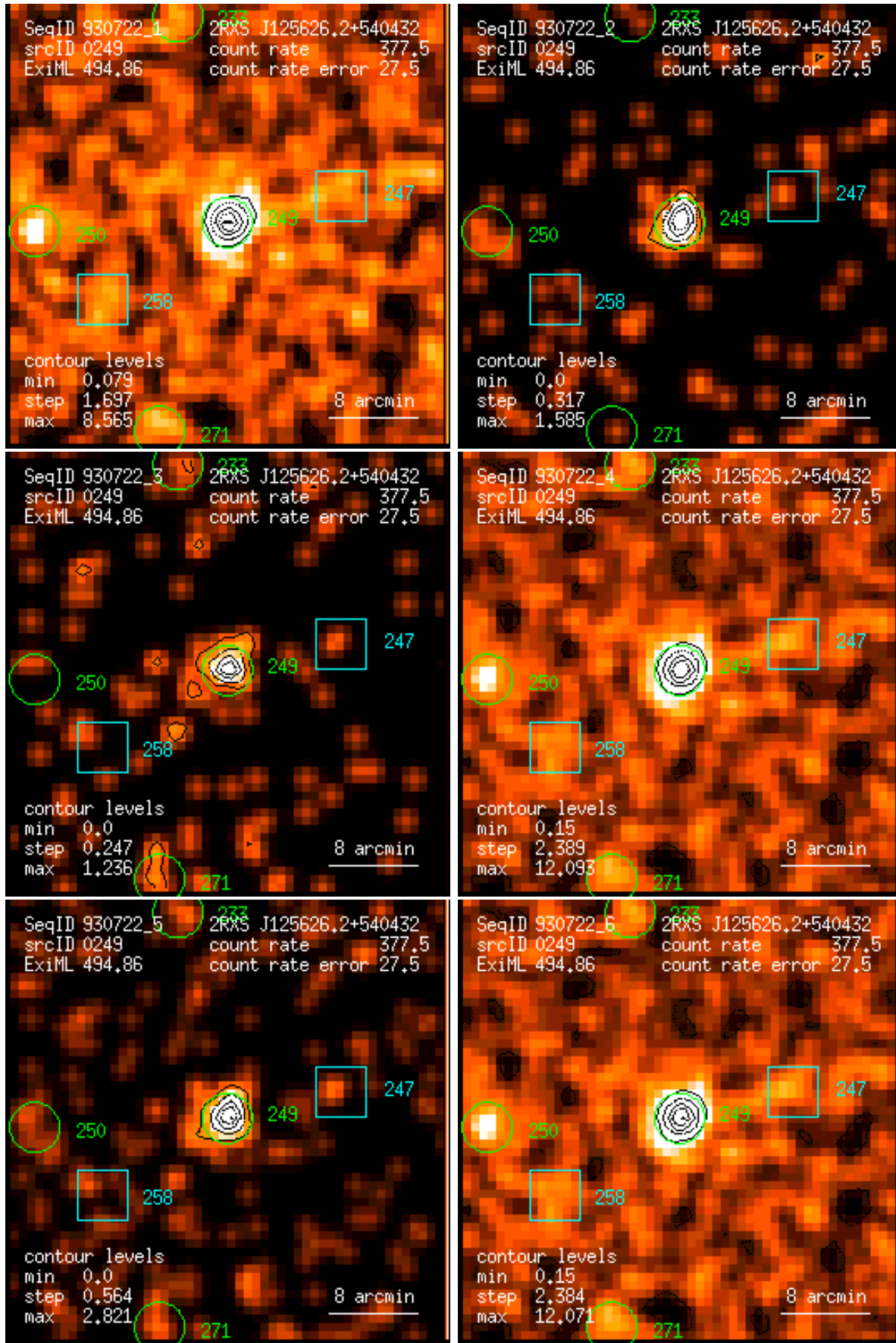
Figure 249: RASS 930722: detection 0249: band rate images, Gaussian filter: (1) PSPC channels 11 – 41, (2) 52 – 90, (3) 91 – 201, (4) 11 – 235, (5) 52 – 201, (6) 11 – 201. Broad band rates in counts/ks. Band rate contour levels in counts/ks/arcmin 2 .
