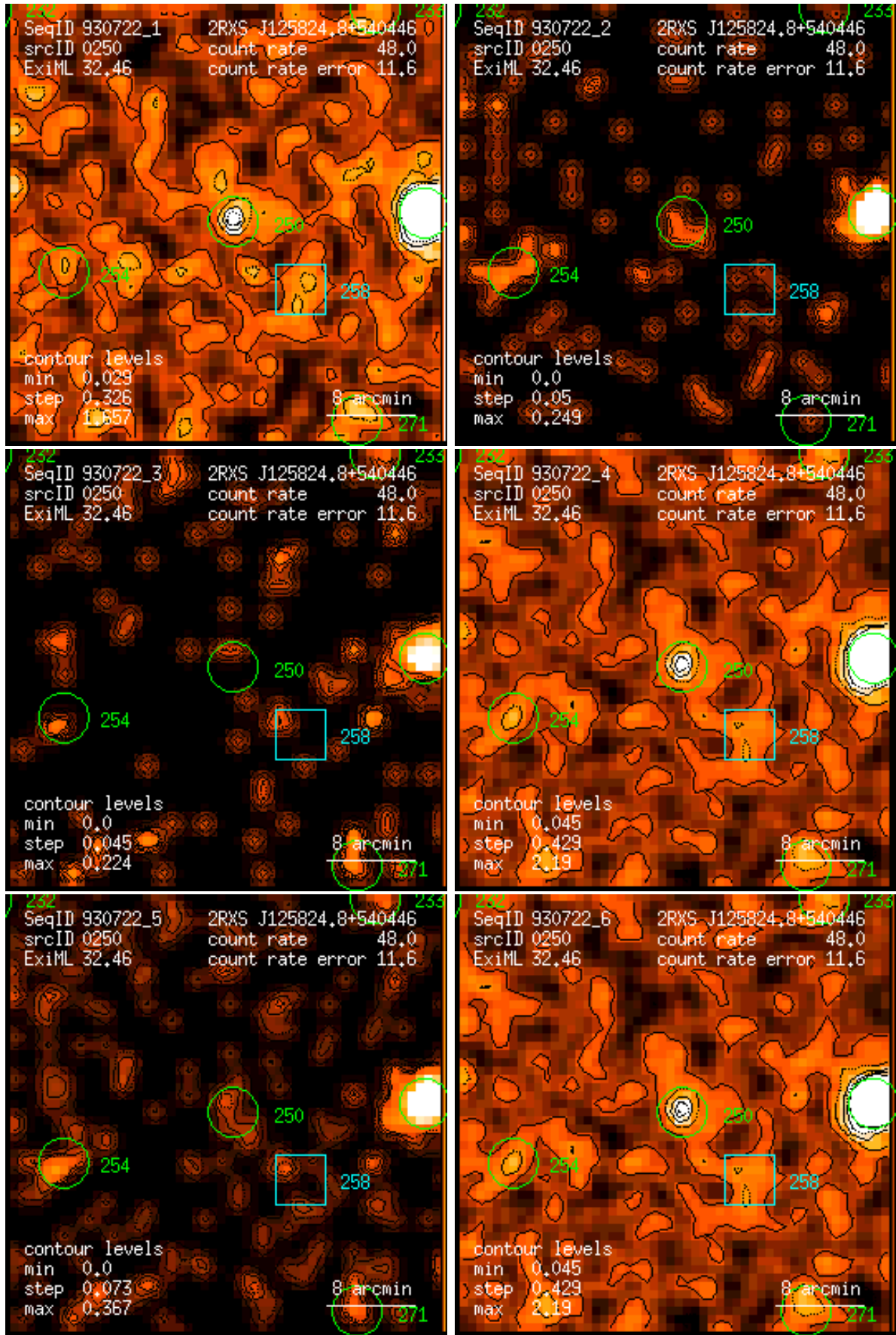
Figure 250: RASS 930722: detection 0250: band rate images, Gaussian filter: (1) PSPC channels 11 – 41, (2) 52 – 90, (3) 91 – 201, (4) 11 – 235, (5) 52 – 201, (6) 11 – 201. Broad band rates in counts/ks. Band rate contour levels in counts/ks/arcmin 2 .
