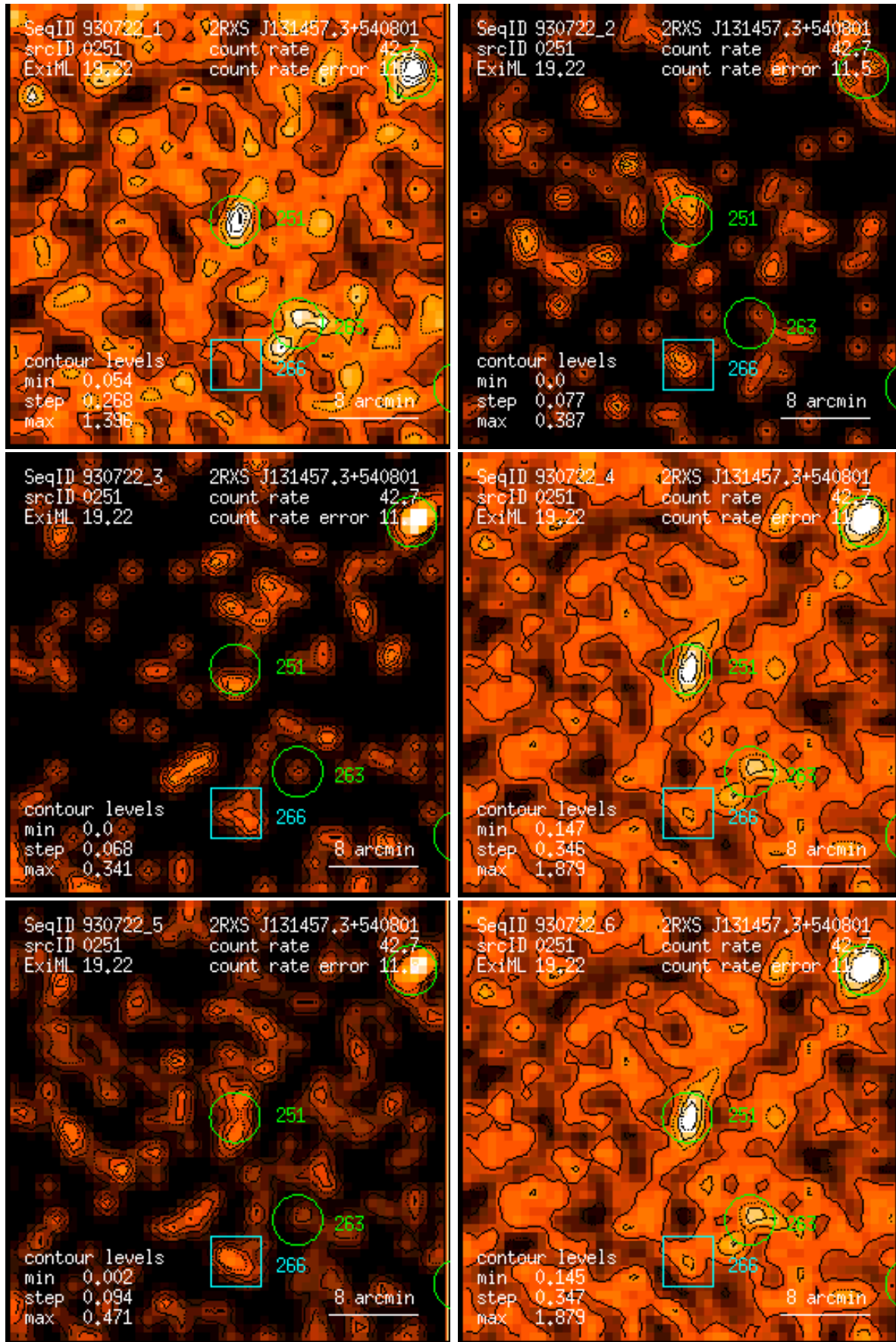
Figure 251: RASS 930722: detection 0251: band rate images, Gaussian filter: (1) PSPC channels 11 – 41, (2) 52 – 90, (3) 91 – 201, (4) 11 – 235, (5) 52 – 201, (6) 11 – 201. Broad band rates in counts/ks. Band rate contour levels in counts/ks/arcmin 2 .
