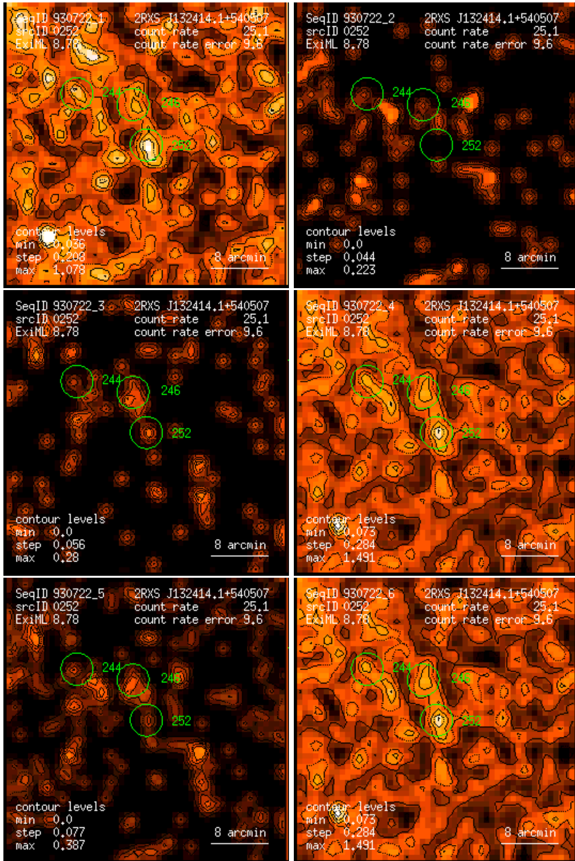
Figure 252: RASS 930722: detection 0252: band rate images, Gaussian filter: (1) PSPC channels 11 – 41, (2) 52 – 90, (3) 91 – 201, (4) 11 – 235, (5) 52 – 201, (6) 11 – 201. Broad band rates in counts/ks. Band rate contour levels in counts/ks/arcmin 2 .
