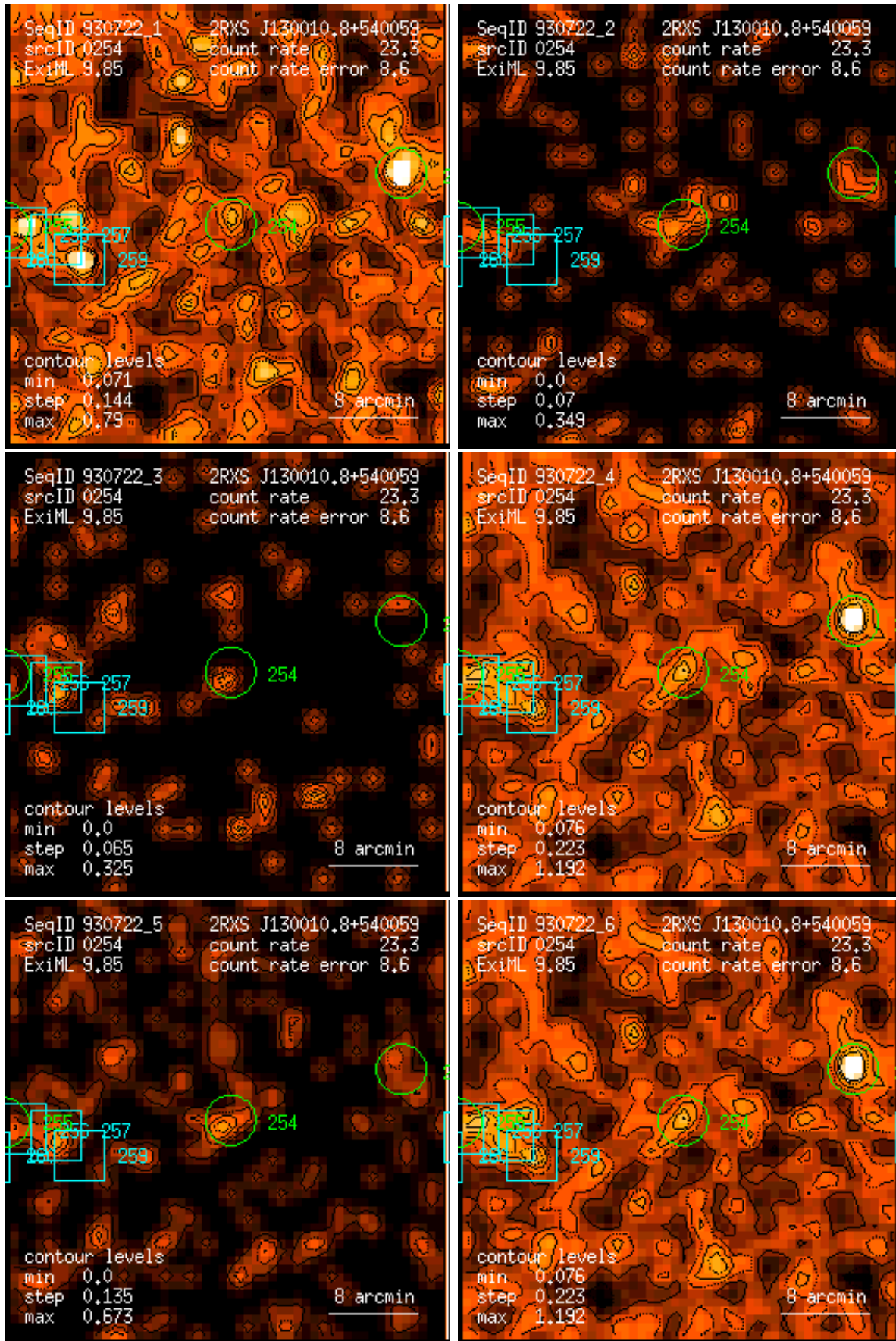
Figure 254: RASS 930722: detection 0254: band rate images, Gaussian filter: (1) PSPC channels 11 – 41, (2) 52 – 90, (3) 91 – 201, (4) 11 – 235, (5) 52 – 201, (6) 11 – 201. Broad band rates in counts/ks. Band rate contour levels in counts/ks/arcmin 2 .
