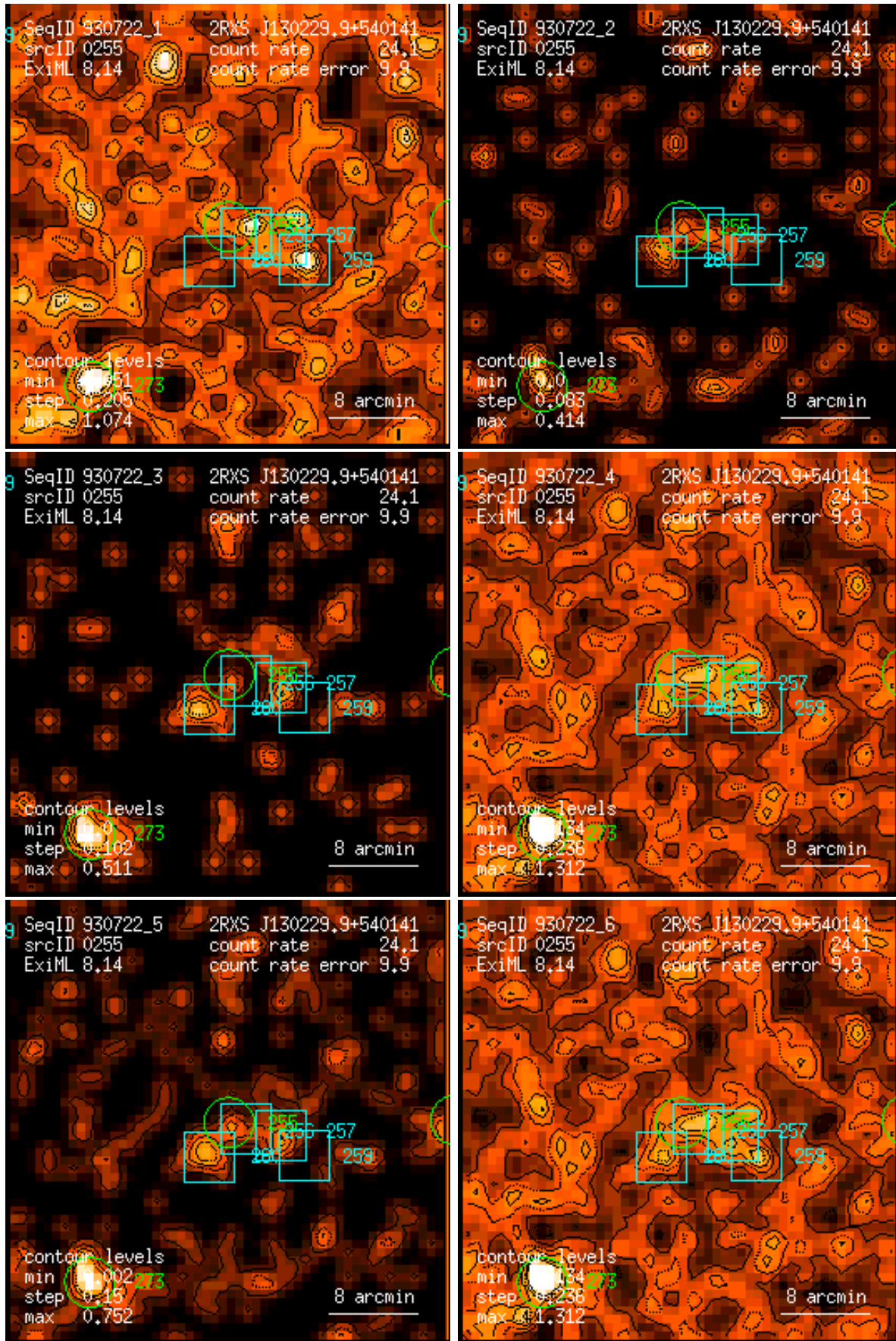
Figure 255: RASS 930722: detection 0255: band rate images, Gaussian filter: (1) PSPC channels 11 – 41, (2) 52 – 90, (3) 91 – 201, (4) 11 – 235, (5) 52 – 201, (6) 11 – 201. Broad band rates in counts/ks. Band rate contour levels in counts/ks/arcmin 2 .
