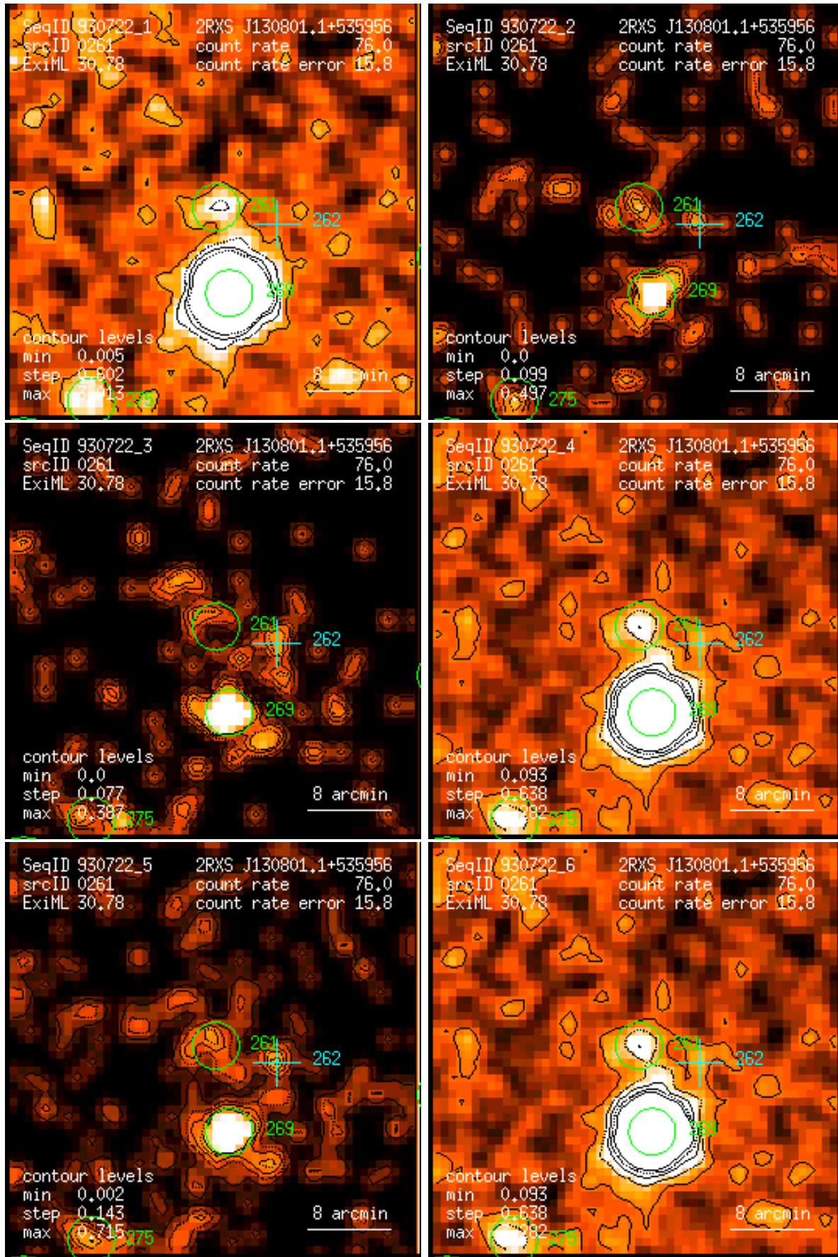
Figure 261: RASS 930722: detection 0261: band rate images, Gaussian filter: (1) PSPC channels 11 – 41, (2) 52 – 90, (3) 91 – 201, (4) 11 – 235, (5) 52 – 201, (6) 11 – 201. Broad band rates in counts/ks. Band rate contour levels in counts/ks/arcmin 2 .
