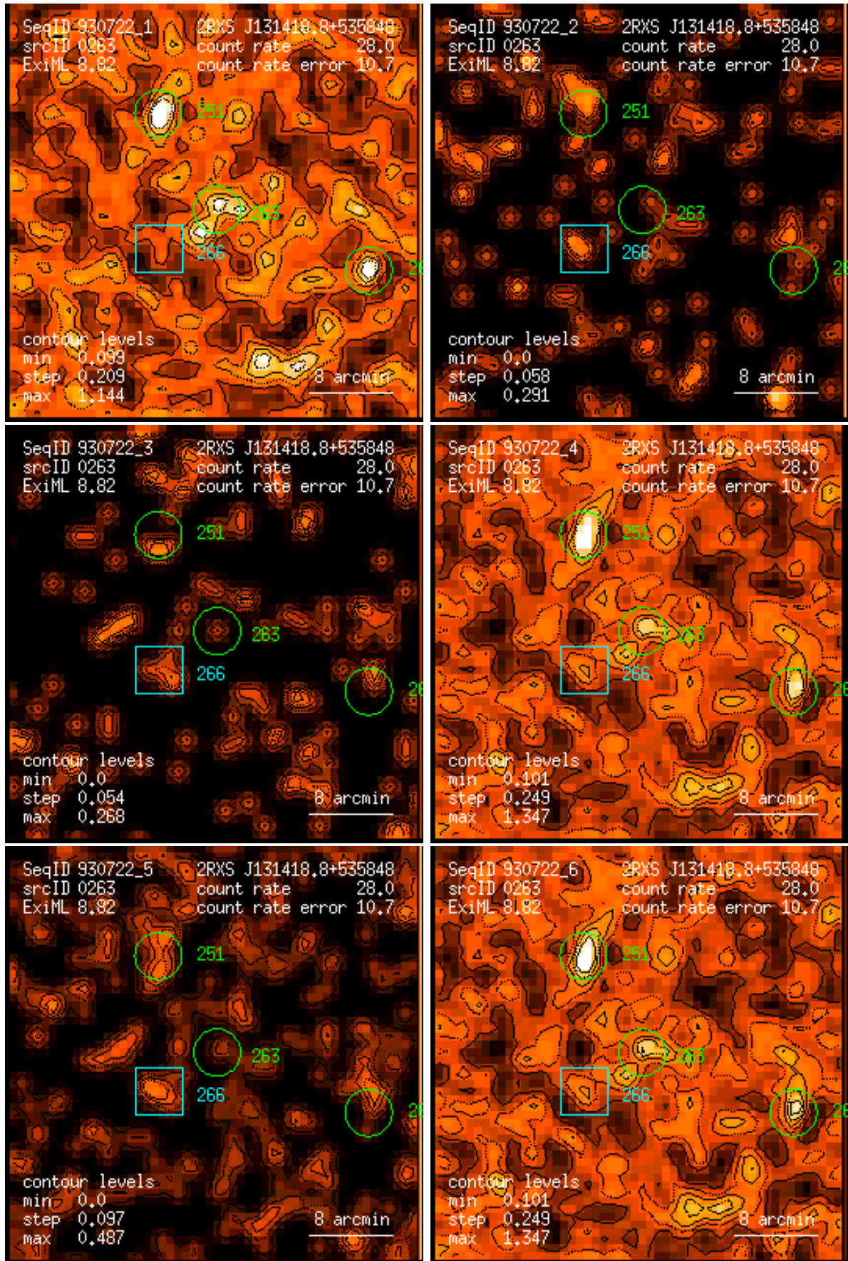
Figure 263: RASS 930722: detection 0263: band rate images, Gaussian filter: (1) PSPC channels 11 – 41, (2) 52 – 90, (3) 91 – 201, (4) 11 – 235, (5) 52 – 201, (6) 11 – 201. Broad band rates in counts/ks. Band rate contour levels in counts/ks/arcmin 2 .
