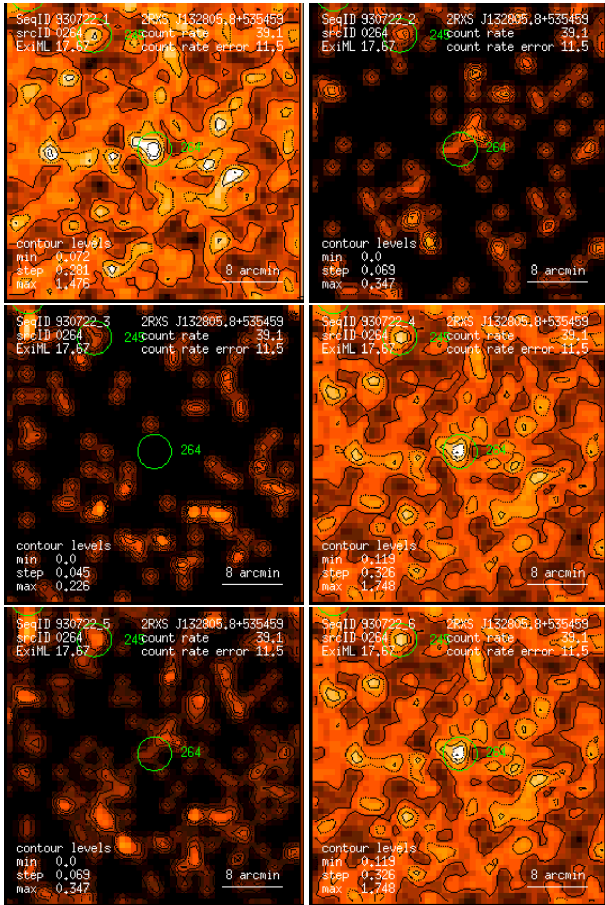
Figure 264: RASS 930722: detection 0264: band rate images, Gaussian filter: (1) PSPC channels 11 – 41, (2) 52 – 90, (3) 91 – 201, (4) 11 – 235, (5) 52 – 201, (6) 11 – 201. Broad band rates in counts/ks. Band rate contour levels in counts/ks/arcmin 2 .
