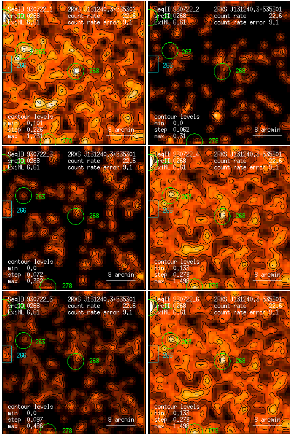
Figure 268: RASS 930722: detection 0268: band rate images, Gaussian filter: (1) PSPC channels 11 – 41, (2) 52 – 90, (3) 91 – 201, (4) 11 – 235, (5) 52 – 201, (6) 11 – 201. Broad band rates in counts/ks. Band rate contour levels in counts/ks/arcmin 2 .
