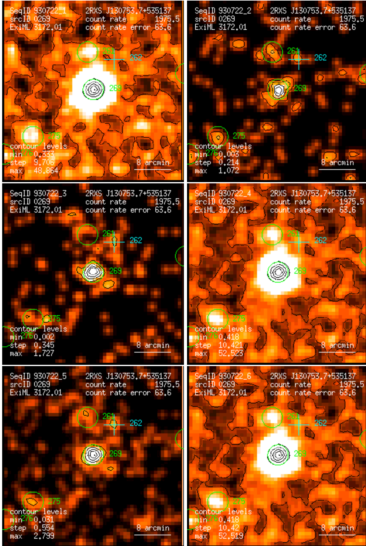
Figure 269: RASS 930722: detection 0269: band rate images, Gaussian filter: (1) PSPC channels 11 – 41, (2) 52 – 90, (3) 91 – 201, (4) 11 – 235, (5) 52 – 201, (6) 11 – 201. Broad band rates in counts/ks. Band rate contour levels in counts/ks/arcmin 2 .
